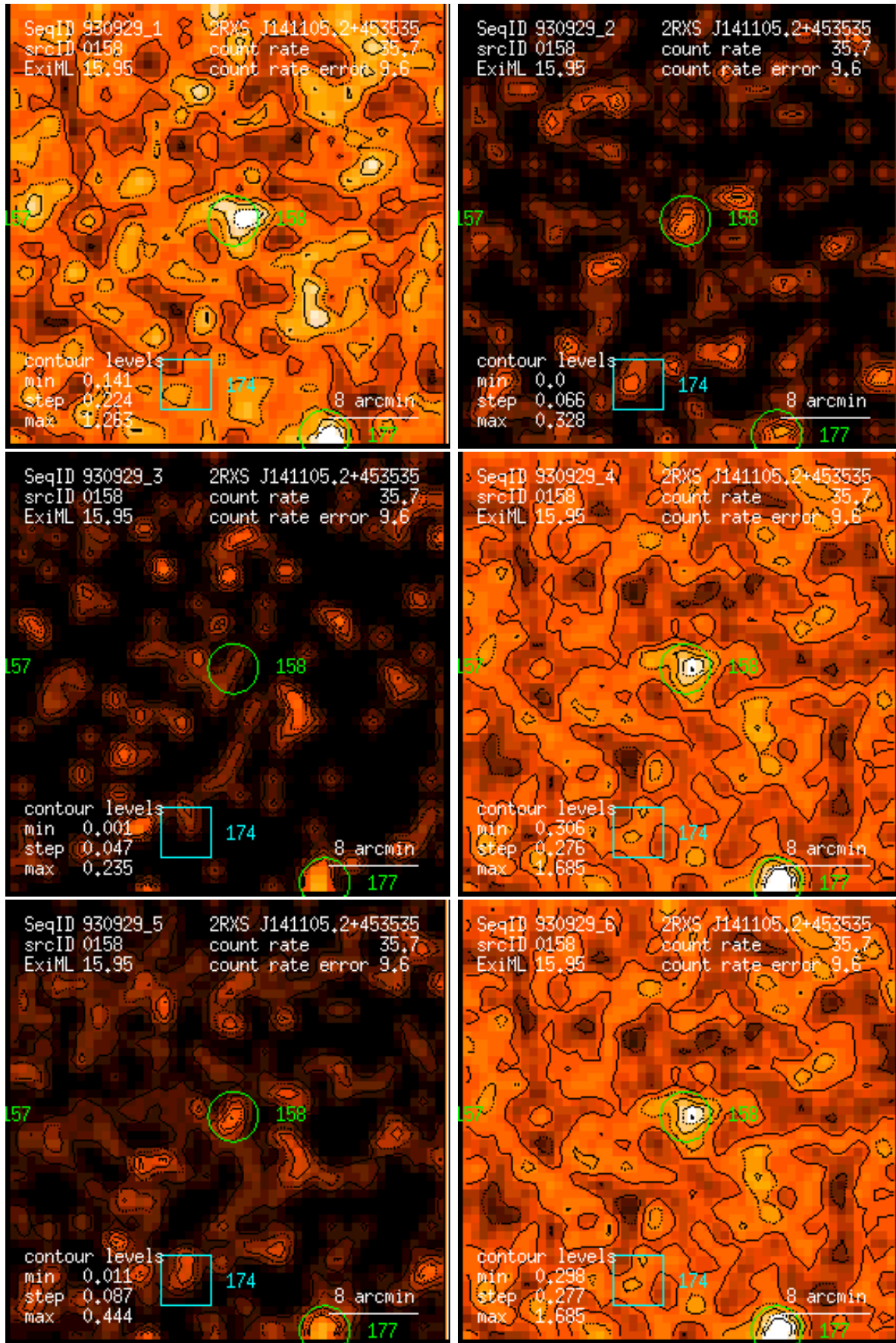
Figure 158: RASS 930929: detection 0158: band rate images, Gaussian filter: (1) PSPC channels 11 – 41, (2) 52 – 90, (3) 91 – 201, (4) 11 – 235, (5) 52 – 201, (6) 11 – 201. Broad band rates in counts/ks. Band rate contour levels in counts/ks/arcmin 2 .
