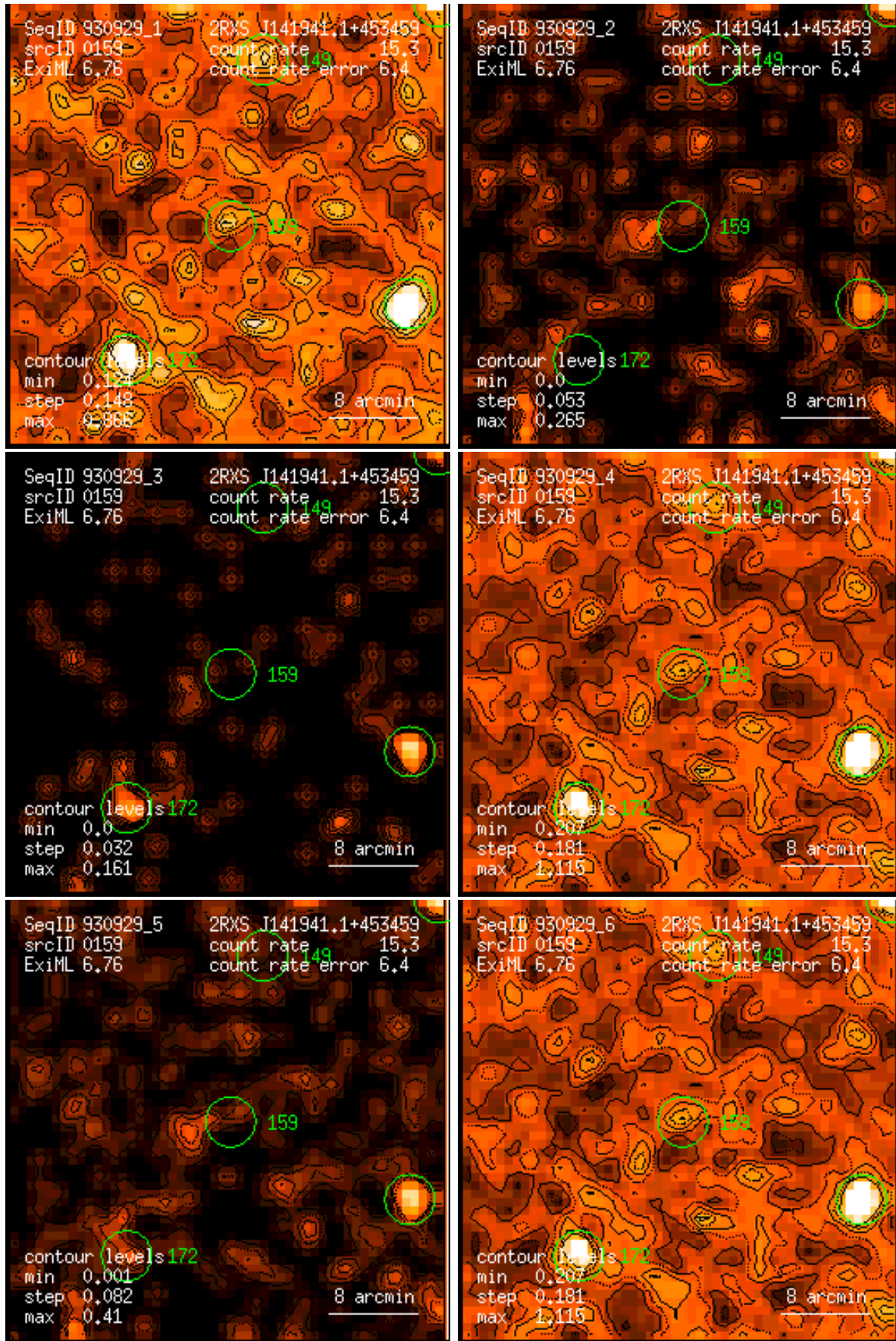
Figure 159: RASS 930929: detection 0159: band rate images, Gaussian filter: (1) PSPC channels 11 – 41, (2) 52 – 90, (3) 91 – 201, (4) 11 – 235, (5) 52 – 201, (6) 11 – 201. Broad band rates in counts/ks. Band rate contour levels in counts/ks/arcmin 2 .
