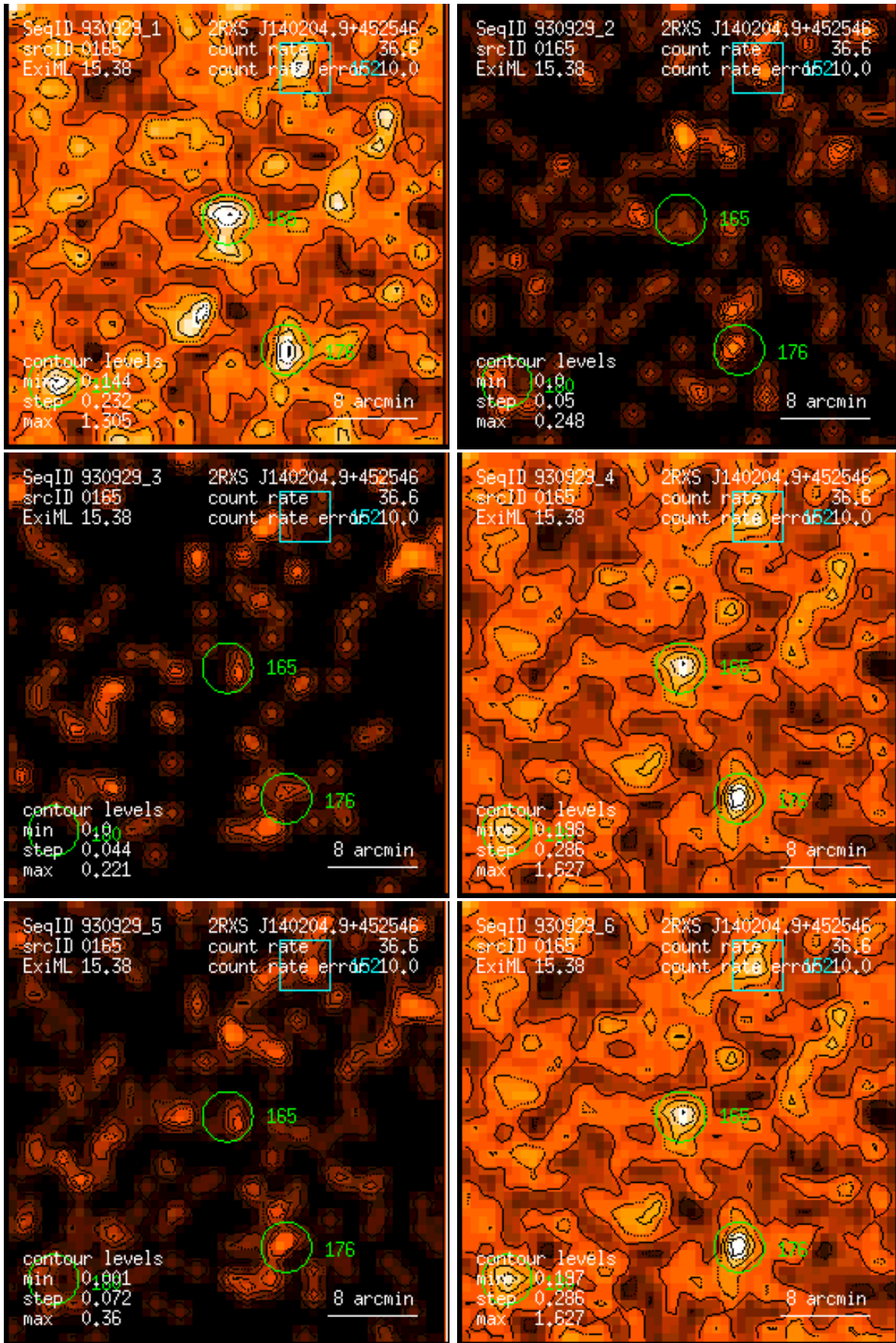
Figure 165: RASS 930929: detection 0165: band rate images, Gaussian filter: (1) PSPC channels 11 – 41, (2) 52 – 90, (3) 91 – 201, (4) 11 – 235, (5) 52 – 201, (6) 11 – 201. Broad band rates in counts/ks. Band rate contour levels in counts/ks/arcmin 2 .
