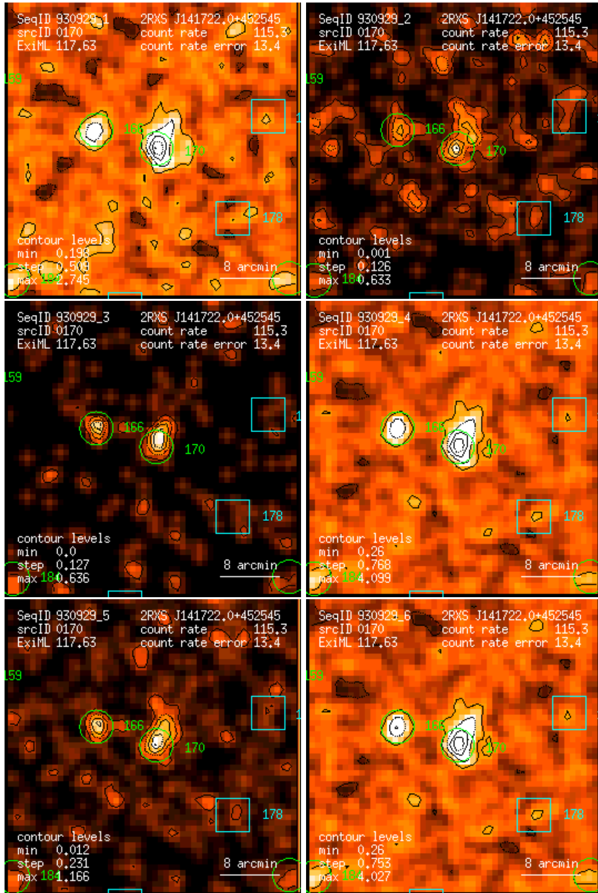
Figure 170: RASS 930929: detection 0170: band rate images, Gaussian filter: (1) PSPC channels 11 – 41, (2) 52 – 90, (3) 91 – 201, (4) 11 – 235, (5) 52 – 201, (6) 11 – 201. Broad band rates in counts/ks. Band rate contour levels in counts/ks/arcmin 2 .
