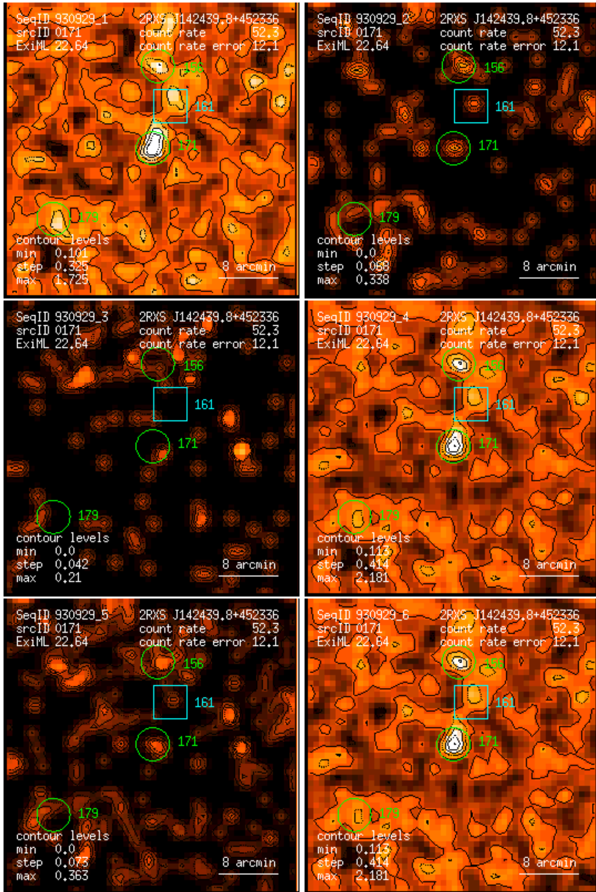
Figure 171: RASS 930929: detection 0171: band rate images, Gaussian filter: (1) PSPC channels 11 – 41, (2) 52 – 90, (3) 91 – 201, (4) 11 – 235, (5) 52 – 201, (6) 11 – 201. Broad band rates in counts/ks. Band rate contour levels in counts/ks/arcmin 2 .
