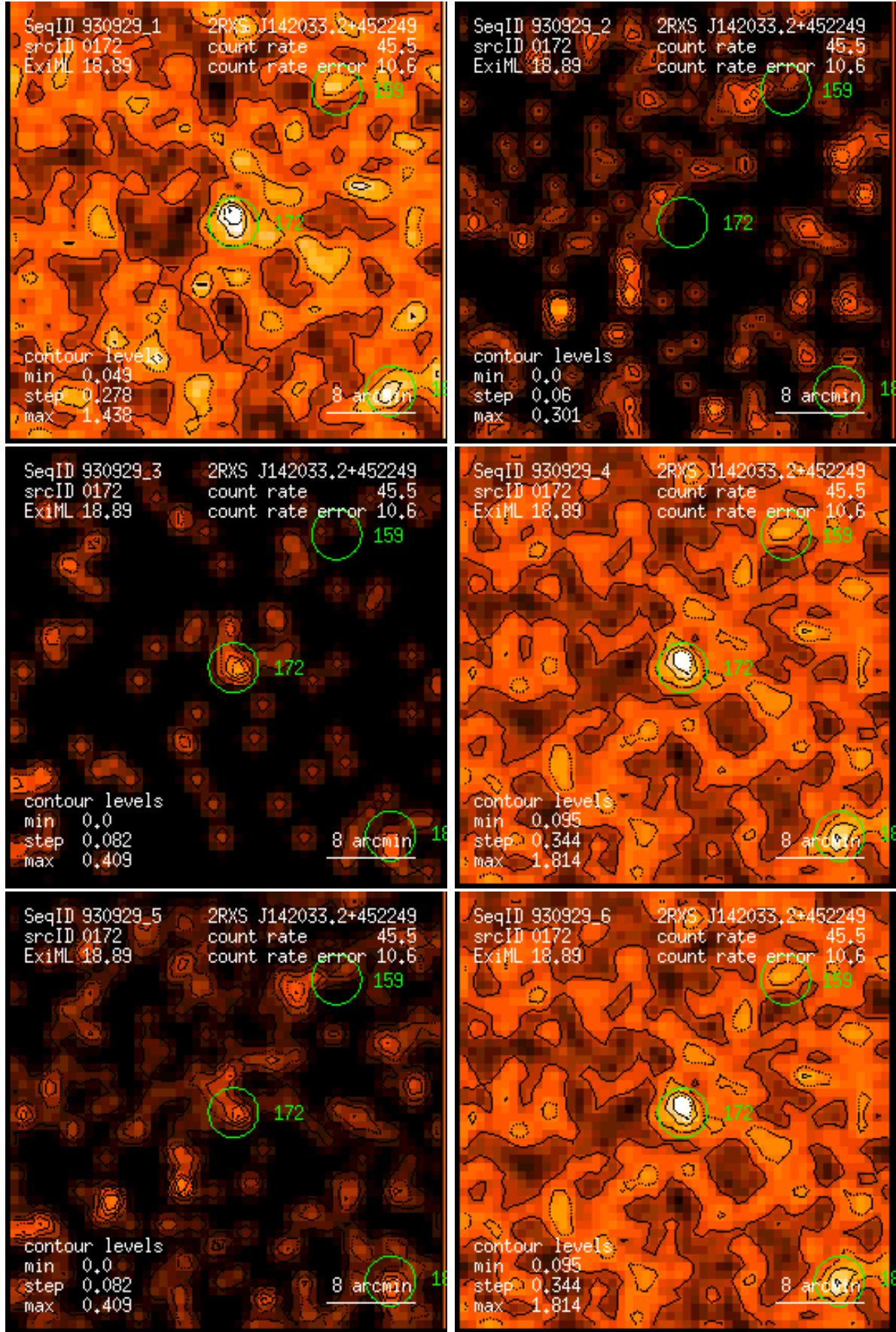
Figure 172: RASS 930929: detection 0172: band rate images, Gaussian filter: (1) PSPC channels 11 – 41, (2) 52 – 90, (3) 91 – 201, (4) 11 – 235, (5) 52 – 201, (6) 11 – 201. Broad band rates in counts/ks. Band rate contour levels in counts/ks/arcmin 2 .
