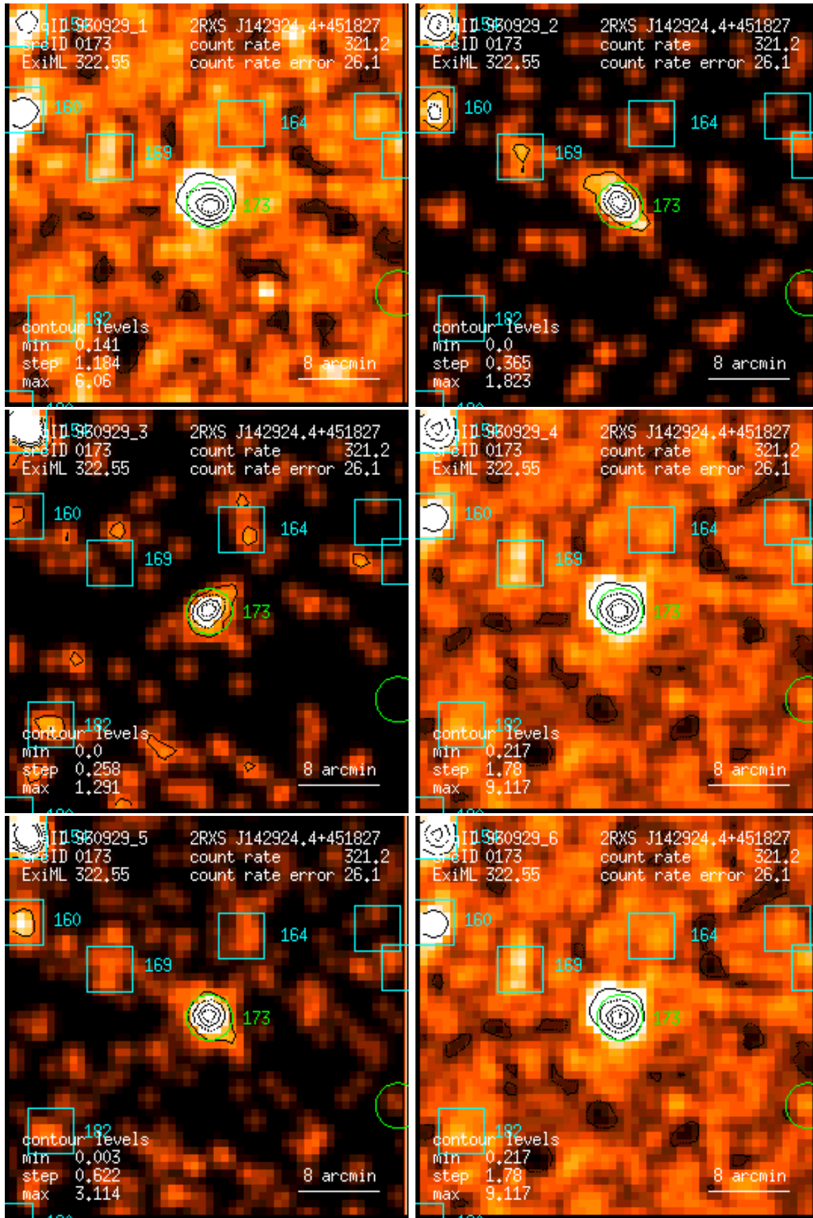
Figure 173: RASS 930929: detection 0173: band rate images, Gaussian filter: (1) PSPC channels 11 – 41, (2) 52 – 90, (3) 91 – 201, (4) 11 – 235, (5) 52 – 201, (6) 11 – 201. Broad band rates in counts/ks. Band rate contour levels in counts/ks/arcmin 2 .
