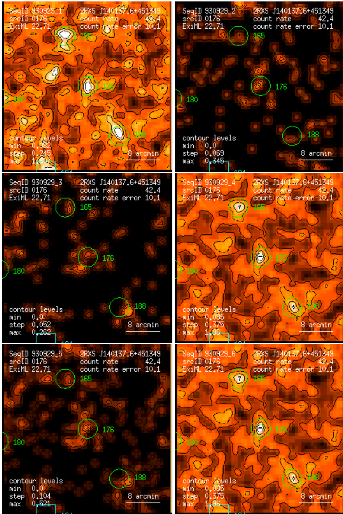
Figure 176: RASS 930929: detection 0176: band rate images, Gaussian filter: (1) PSPC channels 11 – 41, (2) 52 – 90, (3) 91 – 201, (4) 11 – 235, (5) 52 – 201, (6) 11 – 201. Broad band rates in counts/ks. Band rate contour levels in counts/ks/arcmin 2 .
