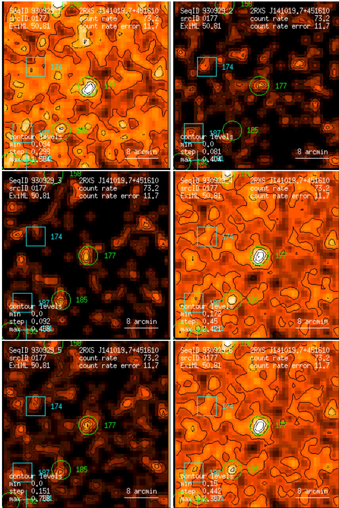
Figure 177: RASS 930929: detection 0177: band rate images, Gaussian filter: (1) PSPC channels 11 – 41, (2) 52 – 90, (3) 91 – 201, (4) 11 – 235, (5) 52 – 201, (6) 11 – 201. Broad band rates in counts/ks. Band rate contour levels in counts/ks/arcmin 2 .
