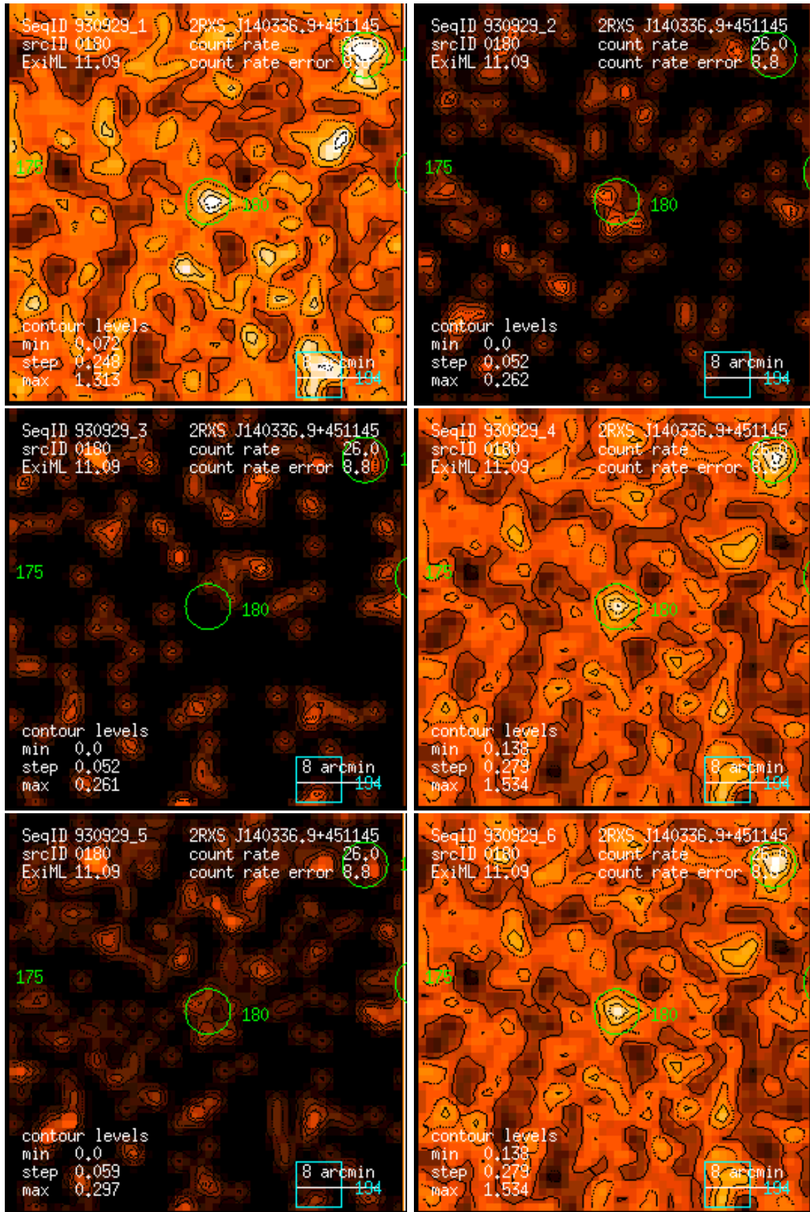
Figure 180: RASS 930929: detection 0180: band rate images, Gaussian filter: (1) PSPC channels 11 – 41, (2) 52 – 90, (3) 91 – 201, (4) 11 – 235, (5) 52 – 201, (6) 11 – 201. Broad band rates in counts/ks. Band rate contour levels in counts/ks/arcmin 2 .
