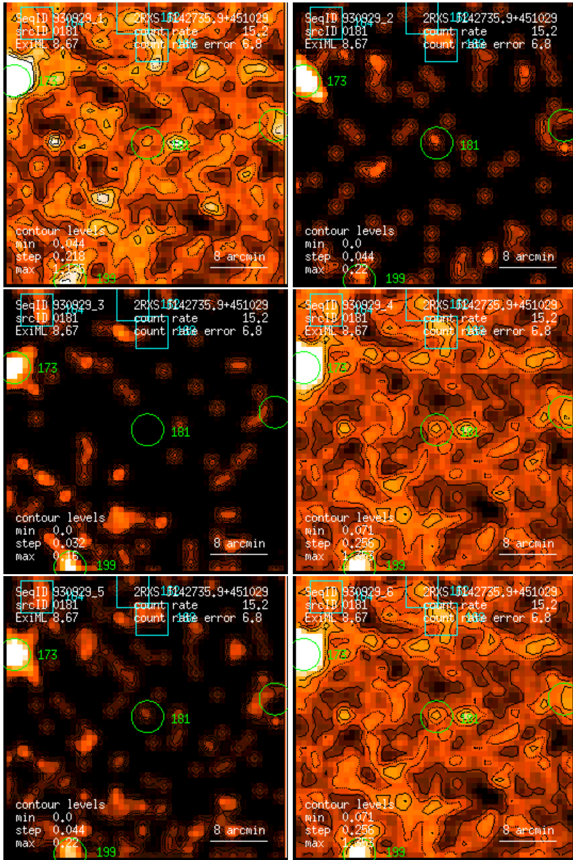
Figure 181: RASS 930929: detection 0181: band rate images, Gaussian filter: (1) PSPC channels 11 – 41, (2) 52 – 90, (3) 91 – 201, (4) 11 – 235, (5) 52 – 201, (6) 11 – 201. Broad band rates in counts/ks. Band rate contour levels in counts/ks/arcmin 2 .
