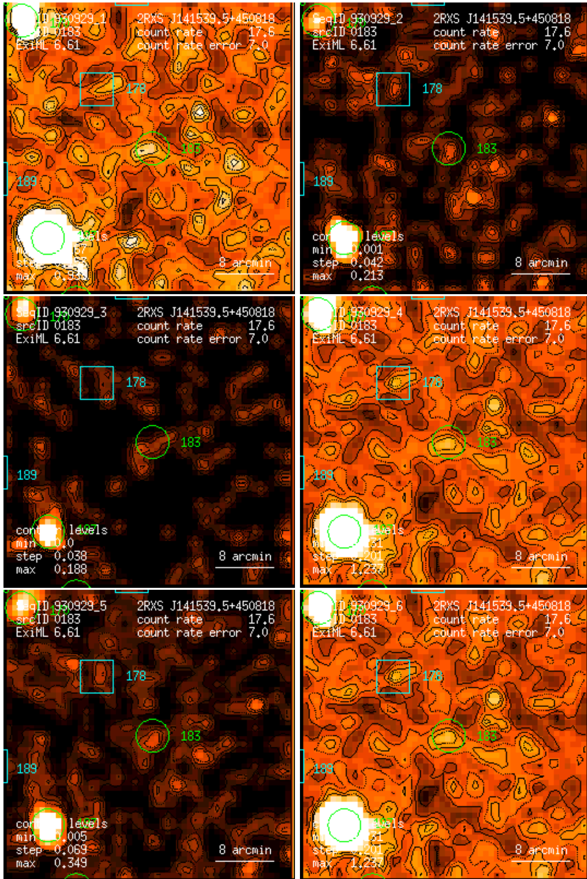
Figure 183: RASS 930929: detection 0183: band rate images, Gaussian filter: (1) PSPC channels 11 – 41, (2) 52 – 90, (3) 91 – 201, (4) 11 – 235, (5) 52 – 201, (6) 11 – 201. Broad band rates in counts/ks. Band rate contour levels in counts/ks/arcmin 2 .
