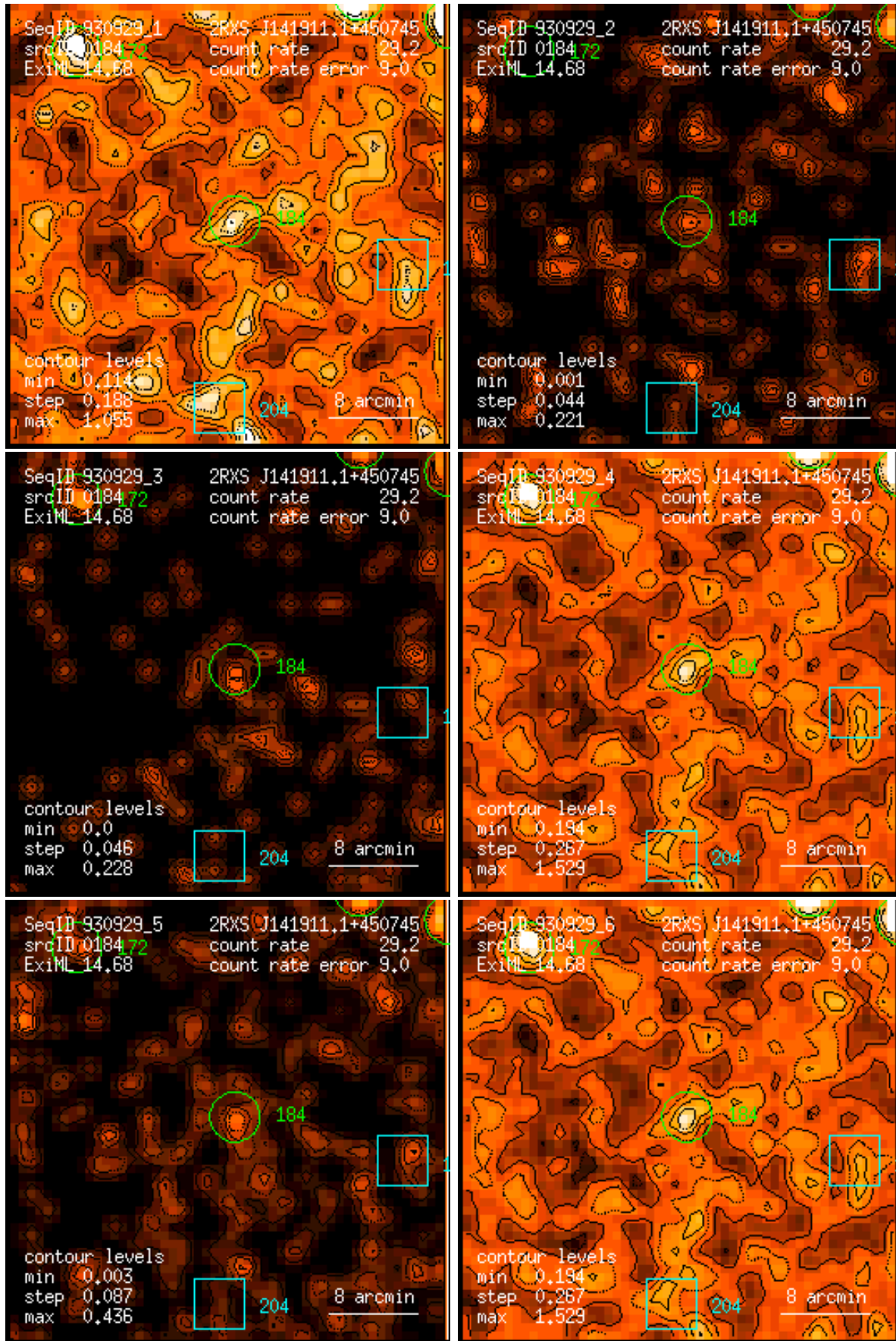
Figure 184: RASS 930929: detection 0184: band rate images, Gaussian filter: (1) PSPC channels 11 – 41, (2) 52 – 90, (3) 91 – 201, (4) 11 – 235, (5) 52 – 201, (6) 11 – 201. Broad band rates in counts/ks. Band rate contour levels in counts/ks/arcmin 2 .
