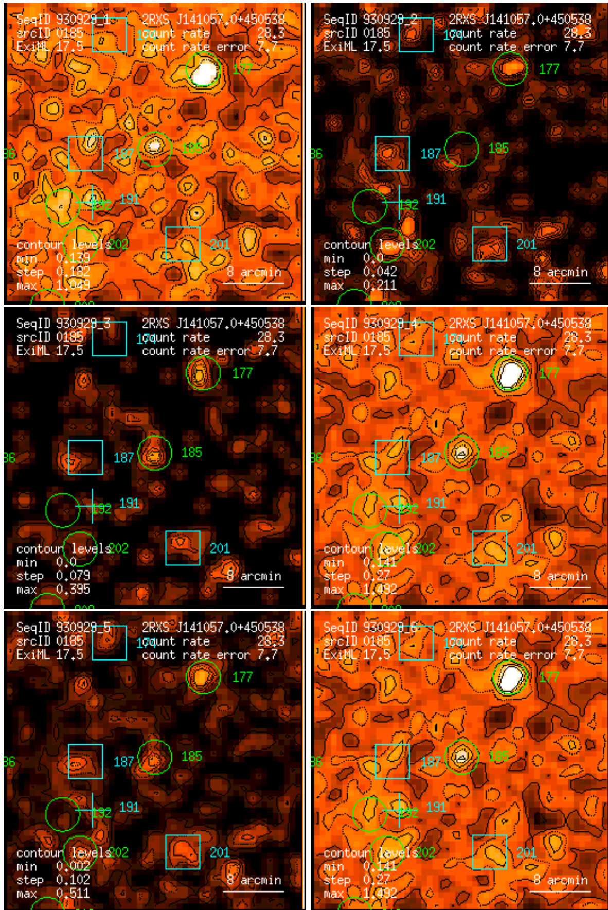
Figure 185: RASS 930929: detection 0185: band rate images, Gaussian filter: (1) PSPC channels 11 – 41, (2) 52 – 90, (3) 91 – 201, (4) 11 – 235, (5) 52 – 201, (6) 11 – 201. Broad band rates in counts/ks. Band rate contour levels in counts/ks/arcmin 2 .
