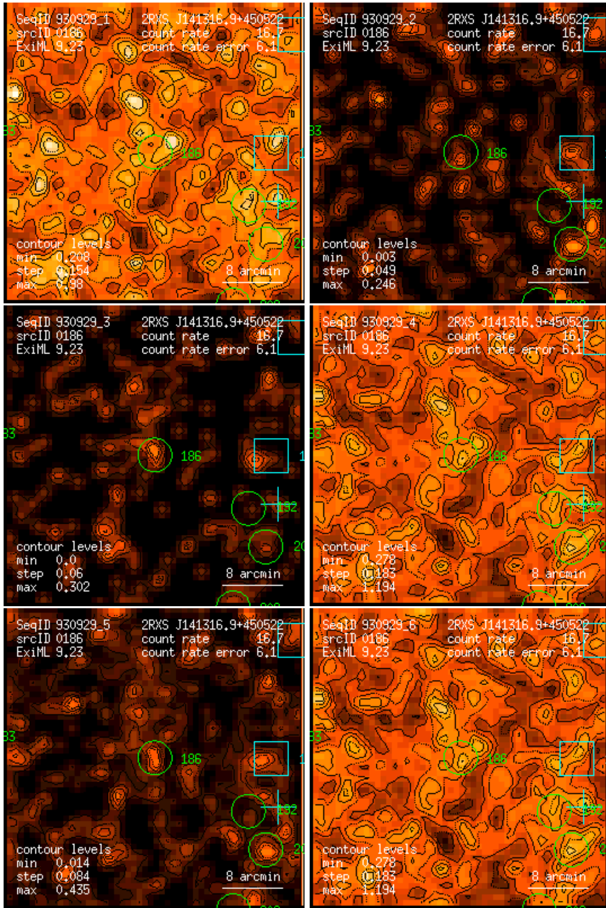
Figure 186: RASS 930929: detection 0186: band rate images, Gaussian filter: (1) PSPC channels 11 – 41, (2) 52 – 90, (3) 91 – 201, (4) 11 – 235, (5) 52 – 201, (6) 11 – 201. Broad band rates in counts/ks. Band rate contour levels in counts/ks/arcmin 2 .
