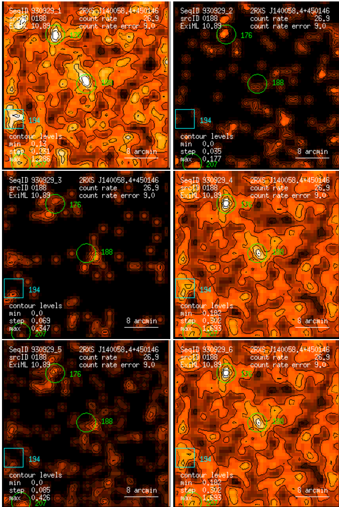
Figure 188: RASS 930929: detection 0188: band rate images, Gaussian filter: (1) PSPC channels 11 – 41, (2) 52 – 90, (3) 91 – 201, (4) 11 – 235, (5) 52 – 201, (6) 11 – 201. Broad band rates in counts/ks. Band rate contour levels in counts/ks/arcmin 2 .
