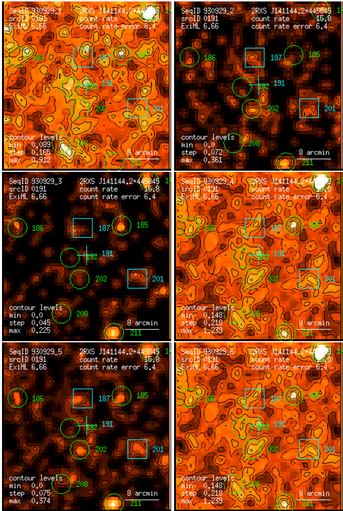
Figure 191: RASS 930929: detection 0191: band rate images, Gaussian filter: (1) PSPC channels 11 – 41, (2) 52 – 90, (3) 91 – 201, (4) 11 – 235, (5) 52 – 201, (6) 11 – 201. Broad band rates in counts/ks. Band rate contour levels in counts/ks/arcmin 2 .
