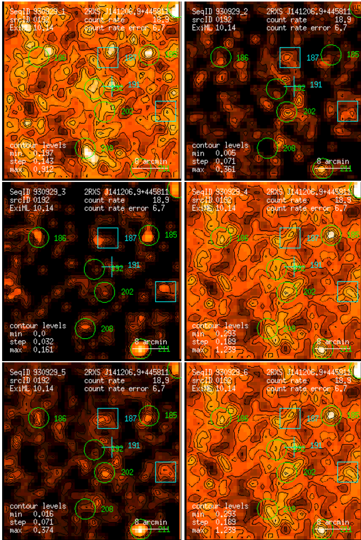
Figure 192: RASS 930929: detection 0192: band rate images, Gaussian filter: (1) PSPC channels 11 – 41, (2) 52 – 90, (3) 91 – 201, (4) 11 – 235, (5) 52 – 201, (6) 11 – 201. Broad band rates in counts/ks. Band rate contour levels in counts/ks/arcmin 2 .
