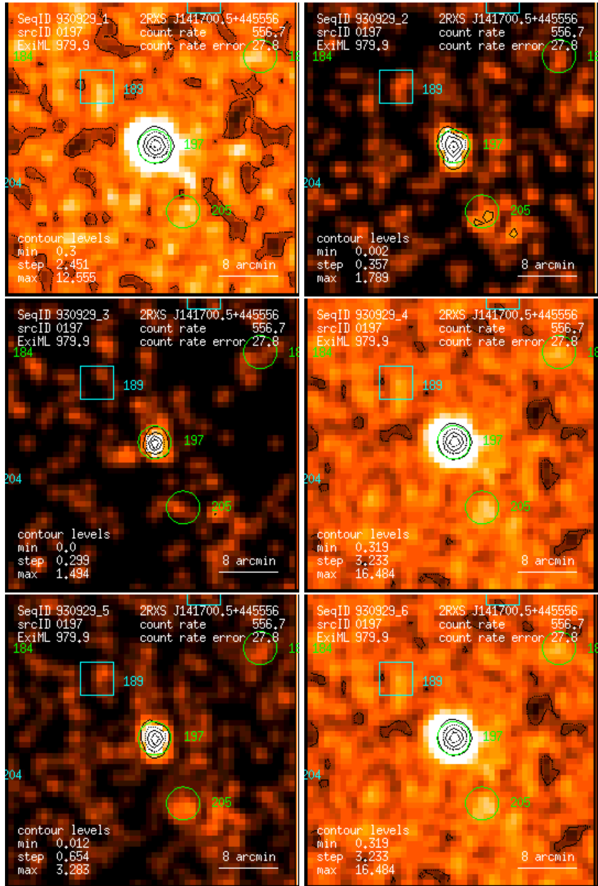
Figure 197: RASS 930929: detection 0197: band rate images, Gaussian filter: (1) PSPC channels 11 – 41, (2) 52 – 90, (3) 91 – 201, (4) 11 – 235, (5) 52 – 201, (6) 11 – 201. Broad band rates in counts/ks. Band rate contour levels in counts/ks/arcmin 2 .
