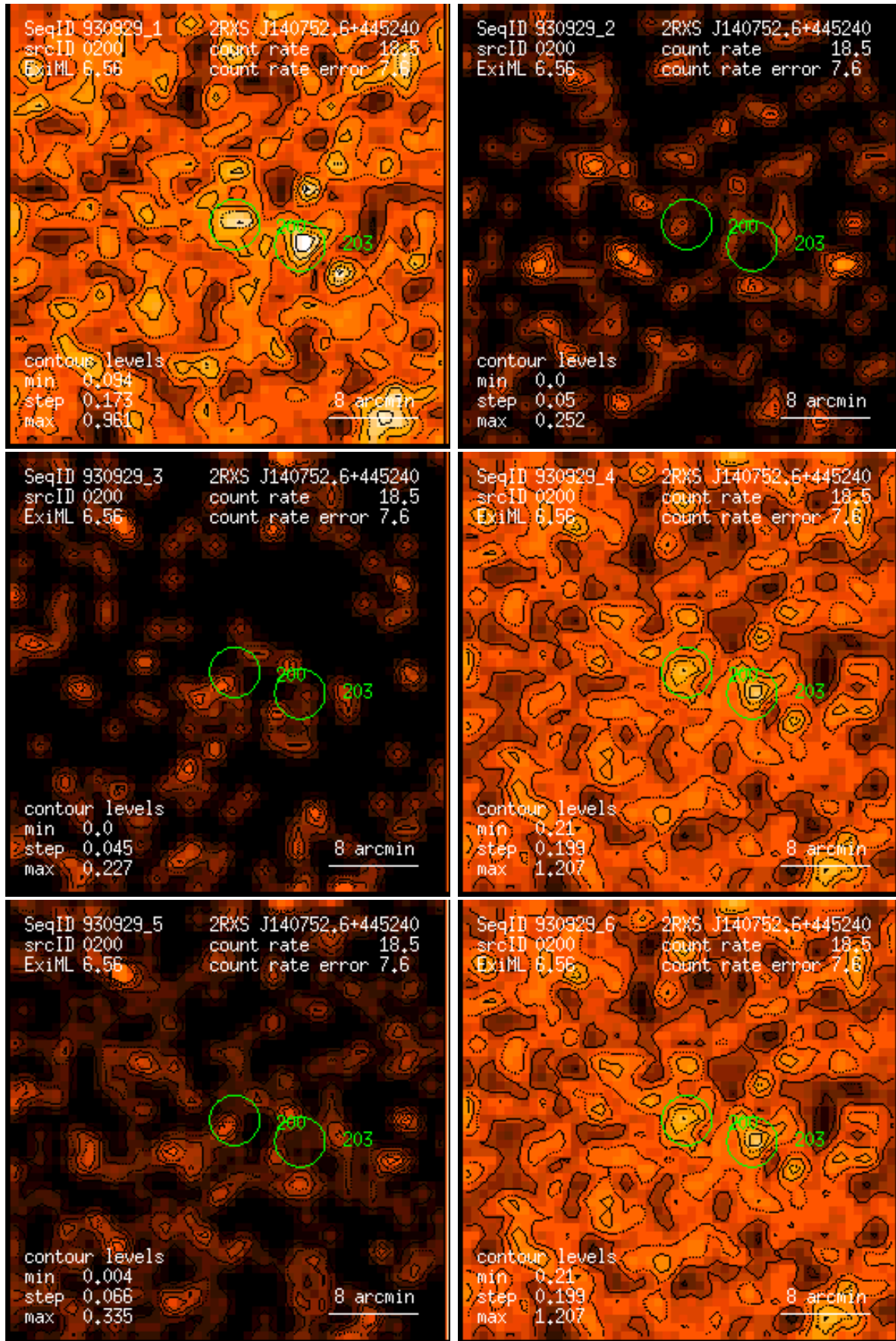
Figure 200: RASS 930929: detection 0200: band rate images, Gaussian filter: (1) PSPC channels 11 – 41, (2) 52 – 90, (3) 91 – 201, (4) 11 – 235, (5) 52 – 201, (6) 11 – 201. Broad band rates in counts/ks. Band rate contour levels in counts/ks/arcmin 2 .
