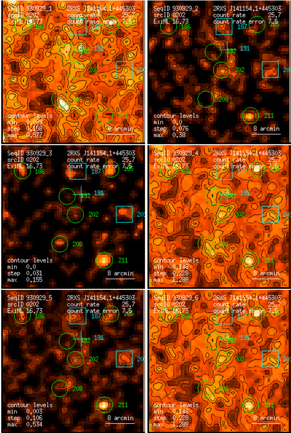
Figure 202: RASS 930929: detection 0202: band rate images, Gaussian filter: (1) PSPC channels 11 – 41, (2) 52 – 90, (3) 91 – 201, (4) 11 – 235, (5) 52 – 201, (6) 11 – 201. Broad band rates in counts/ks. Band rate contour levels in counts/ks/arcmin 2 .
