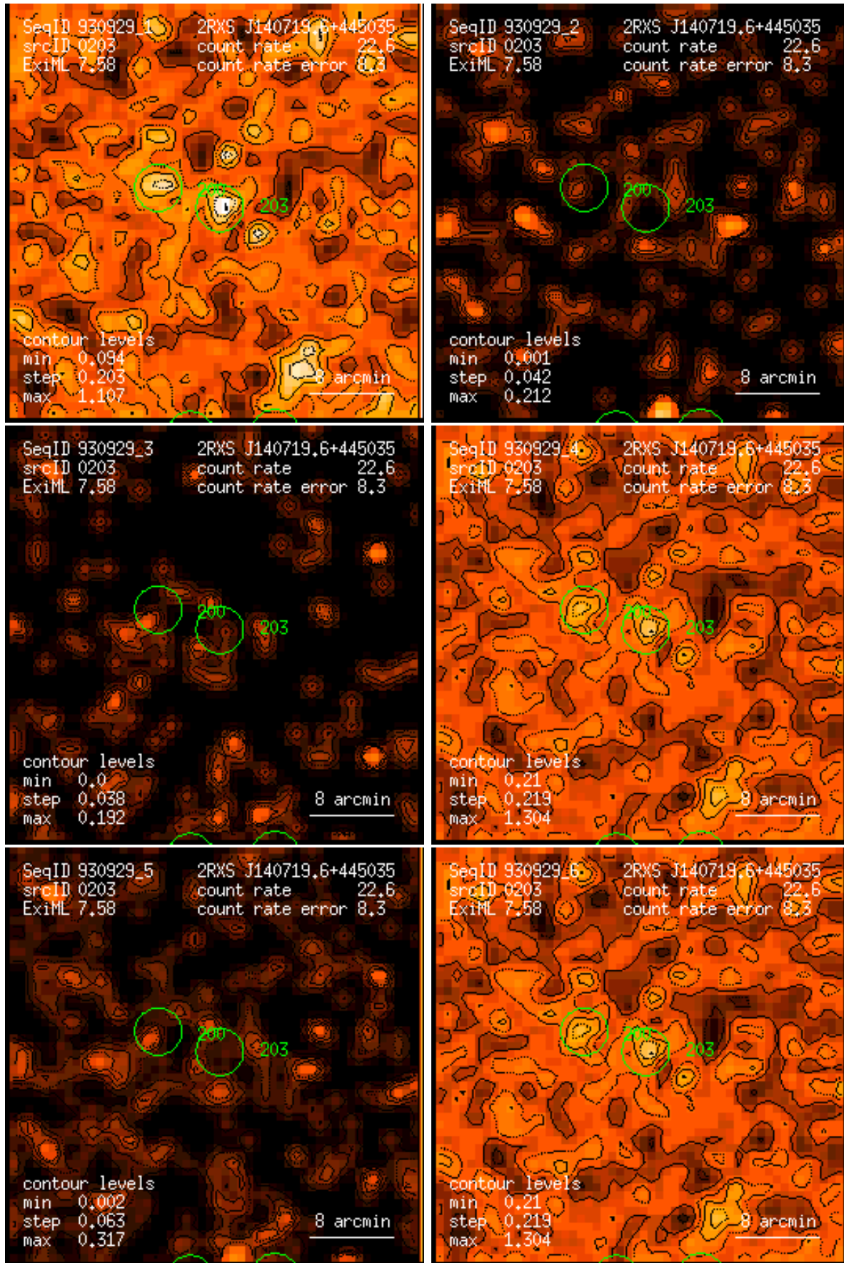
Figure 203: RASS 930929: detection 0203: band rate images, Gaussian filter: (1) PSPC channels 11 – 41, (2) 52 – 90, (3) 91 – 201, (4) 11 – 235, (5) 52 – 201, (6) 11 – 201. Broad band rates in counts/ks. Band rate contour levels in counts/ks/arcmin 2 .
