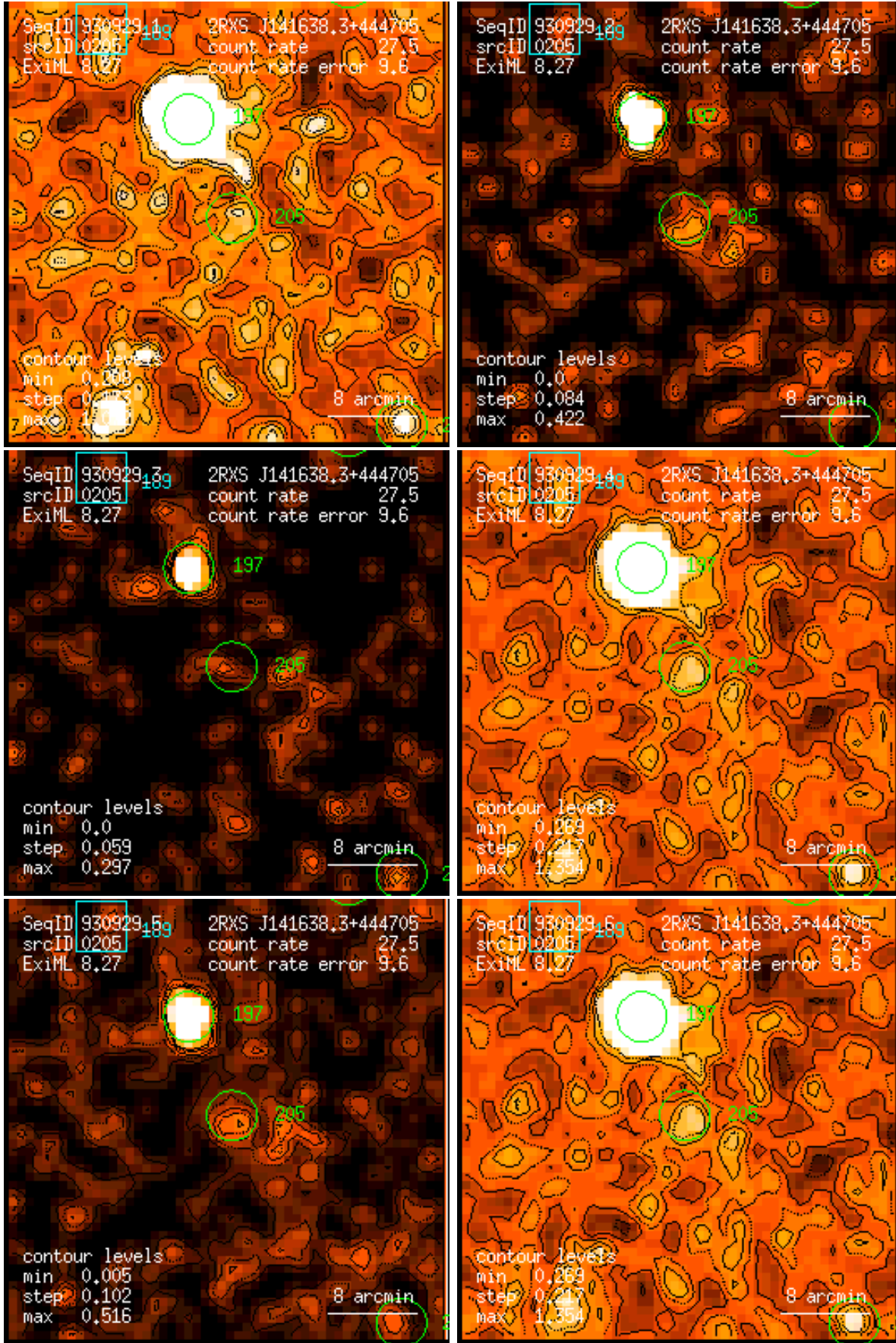
Figure 205: RASS 930929: detection 0205: band rate images, Gaussian filter: (1) PSPC channels 11 – 41, (2) 52 – 90, (3) 91 – 201, (4) 11 – 235, (5) 52 – 201, (6) 11 – 201. Broad band rates in counts/ks. Band rate contour levels in counts/ks/arcmin 2 .
