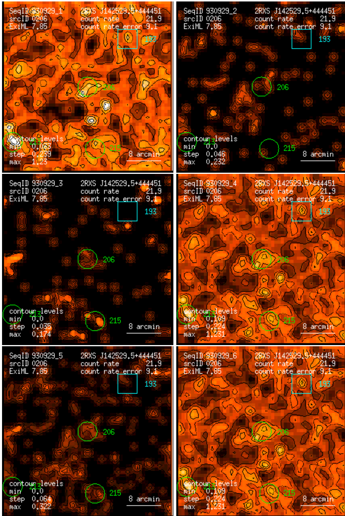
Figure 206: RASS 930929: detection 0206: band rate images, Gaussian filter: (1) PSPC channels 11 – 41, (2) 52 – 90, (3) 91 – 201, (4) 11 – 235, (5) 52 – 201, (6) 11 – 201. Broad band rates in counts/ks. Band rate contour levels in counts/ks/arcmin 2 .
