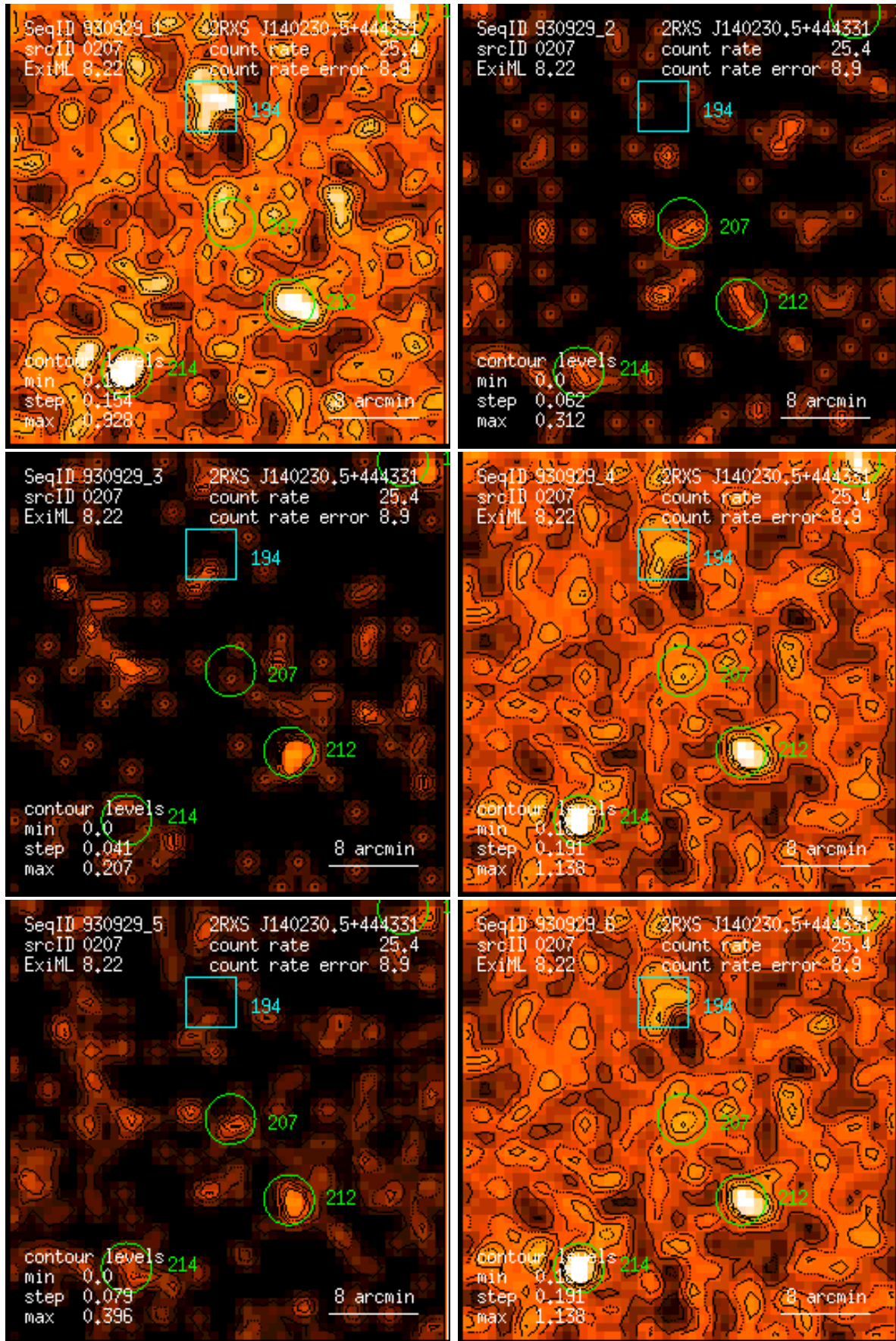
Figure 207: RASS 930929: detection 0207: band rate images, Gaussian filter: (1) PSPC channels 11 – 41, (2) 52 – 90, (3) 91 – 201, (4) 11 – 235, (5) 52 – 201, (6) 11 – 201. Broad band rates in counts/ks. Band rate contour levels in counts/ks/arcmin 2 .
