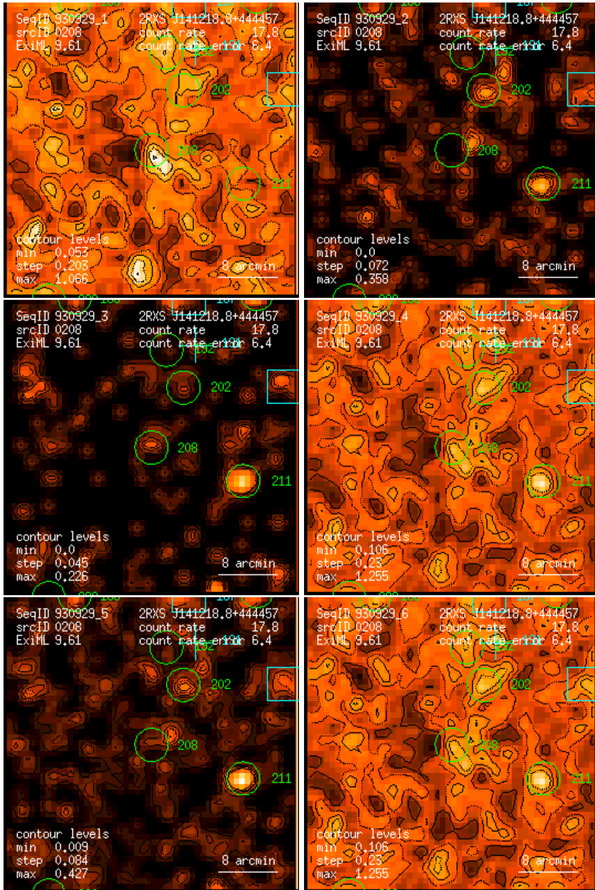
Figure 208: RASS 930929: detection 0208: band rate images, Gaussian filter: (1) PSPC channels 11 – 41, (2) 52 – 90, (3) 91 – 201, (4) 11 – 235, (5) 52 – 201, (6) 11 – 201. Broad band rates in counts/ks. Band rate contour levels in counts/ks/arcmin 2 .
