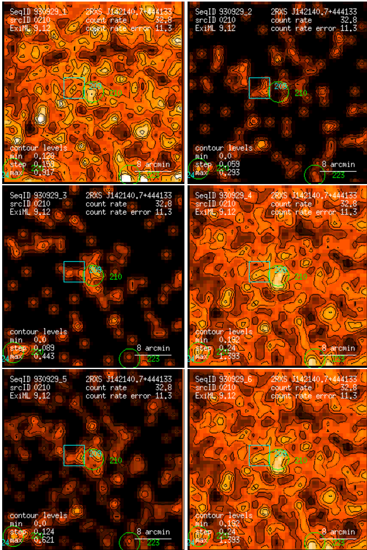
Figure 210: RASS 930929: detection 0210: band rate images, Gaussian filter: (1) PSPC channels 11 – 41, (2) 52 – 90, (3) 91 – 201, (4) 11 – 235, (5) 52 – 201, (6) 11 – 201. Broad band rates in counts/ks. Band rate contour levels in counts/ks/arcmin 2 .
