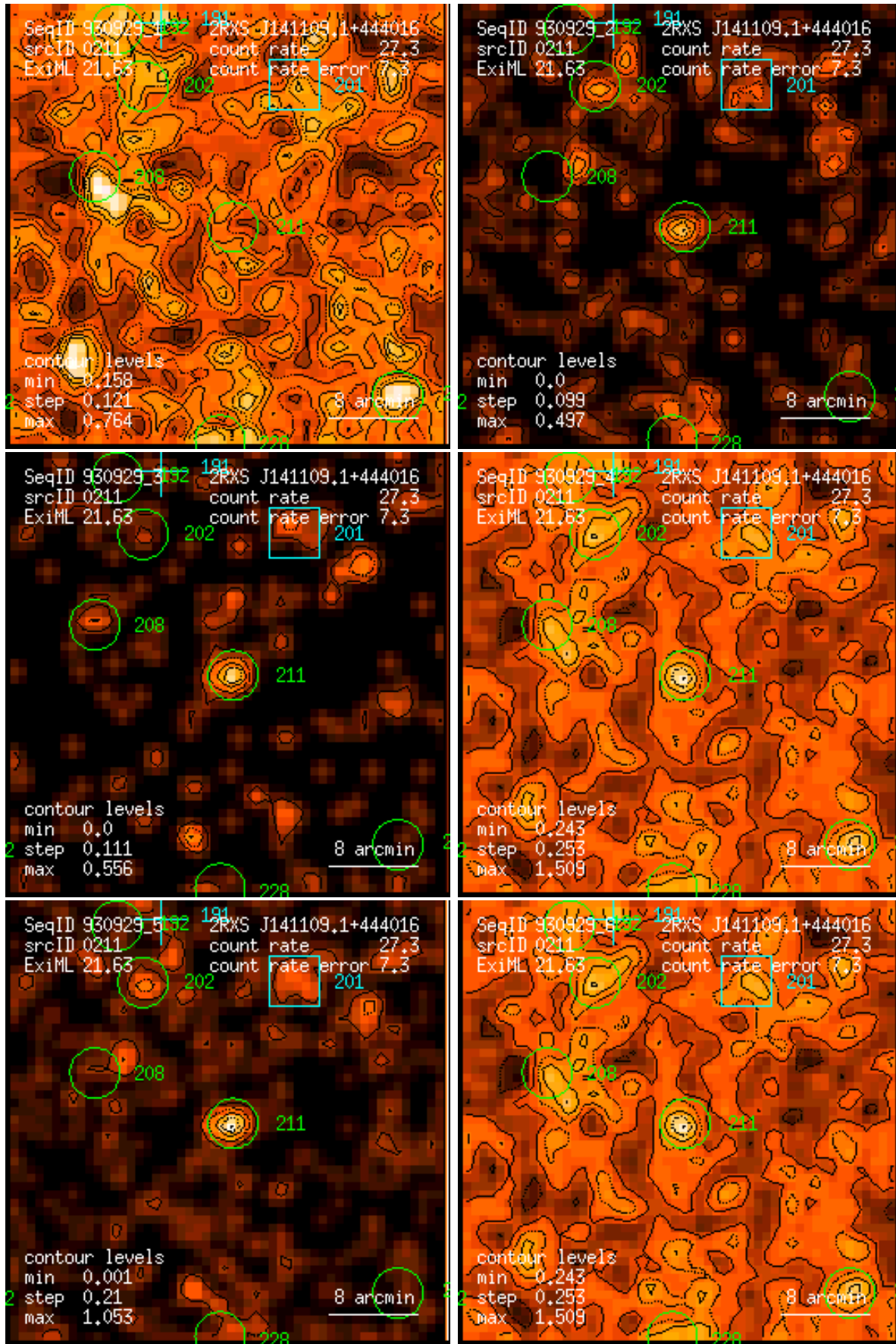
Figure 211: RASS 930929: detection 0211: band rate images, Gaussian filter: (1) PSPC channels 11 – 41, (2) 52 – 90, (3) 91 – 201, (4) 11 – 235, (5) 52 – 201, (6) 11 – 201. Broad band rates in counts/ks. Band rate contour levels in counts/ks/arcmin 2 .
