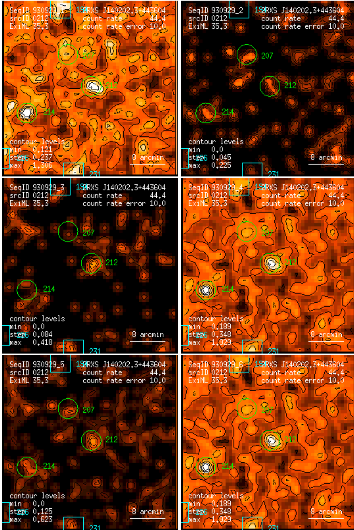
Figure 212: RASS 930929: detection 0212: band rate images, Gaussian filter: (1) PSPC channels 11 – 41, (2) 52 – 90, (3) 91 – 201, (4) 11 – 235, (5) 52 – 201, (6) 11 – 201. Broad band rates in counts/ks. Band rate contour levels in counts/ks/arcmin 2 .
