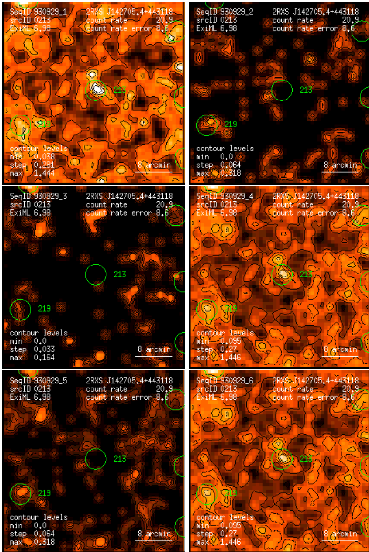
Figure 213: RASS 930929: detection 0213: band rate images, Gaussian filter: (1) PSPC channels 11 – 41, (2) 52 – 90, (3) 91 – 201, (4) 11 – 235, (5) 52 – 201, (6) 11 – 201. Broad band rates in counts/ks. Band rate contour levels in counts/ks/arcmin 2 .
