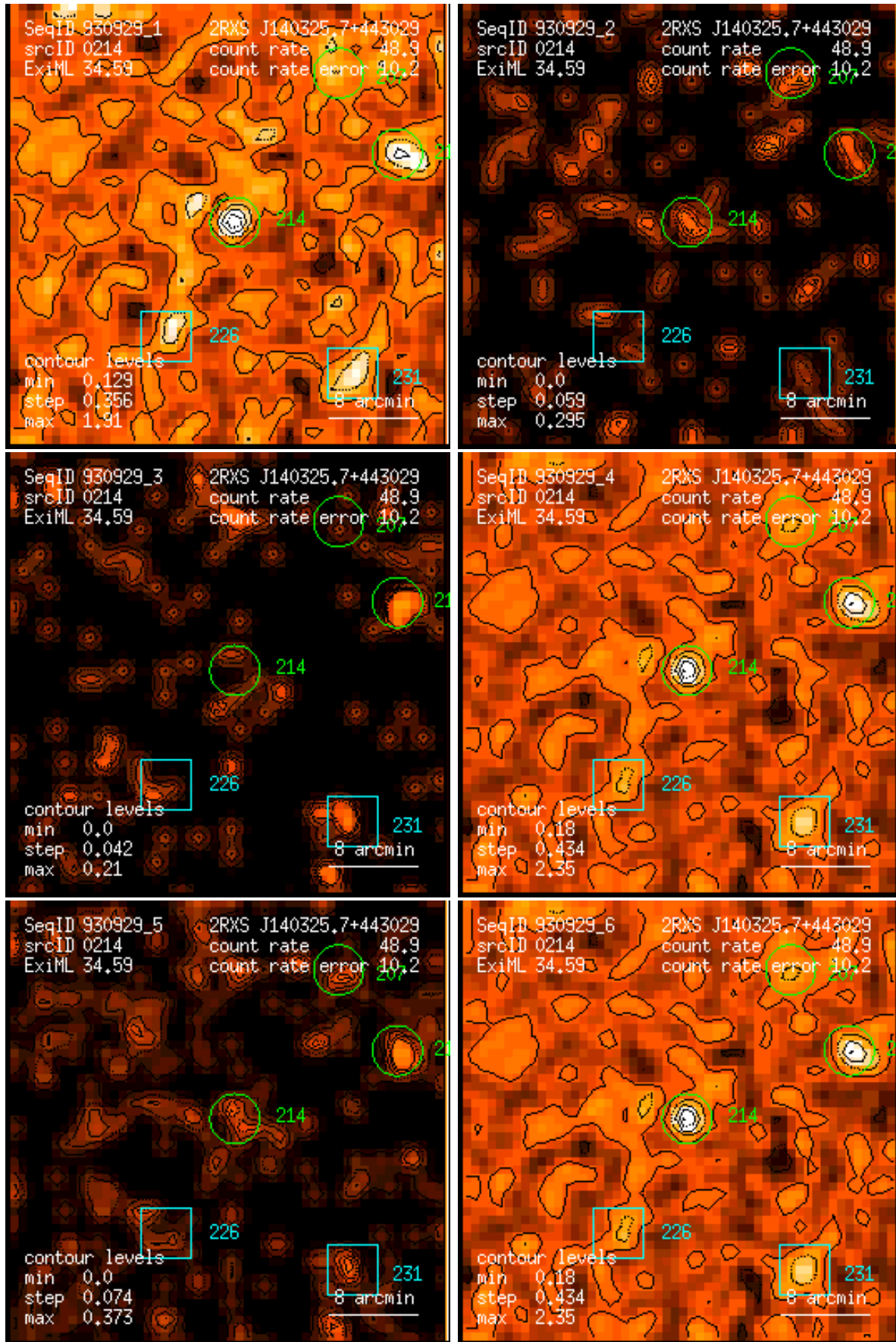
Figure 214: RASS 930929: detection 0214: band rate images, Gaussian filter: (1) PSPC channels 11 – 41, (2) 52 – 90, (3) 91 – 201, (4) 11 – 235, (5) 52 – 201, (6) 11 – 201. Broad band rates in counts/ks. Band rate contour levels in counts/ks/arcmin 2 .
