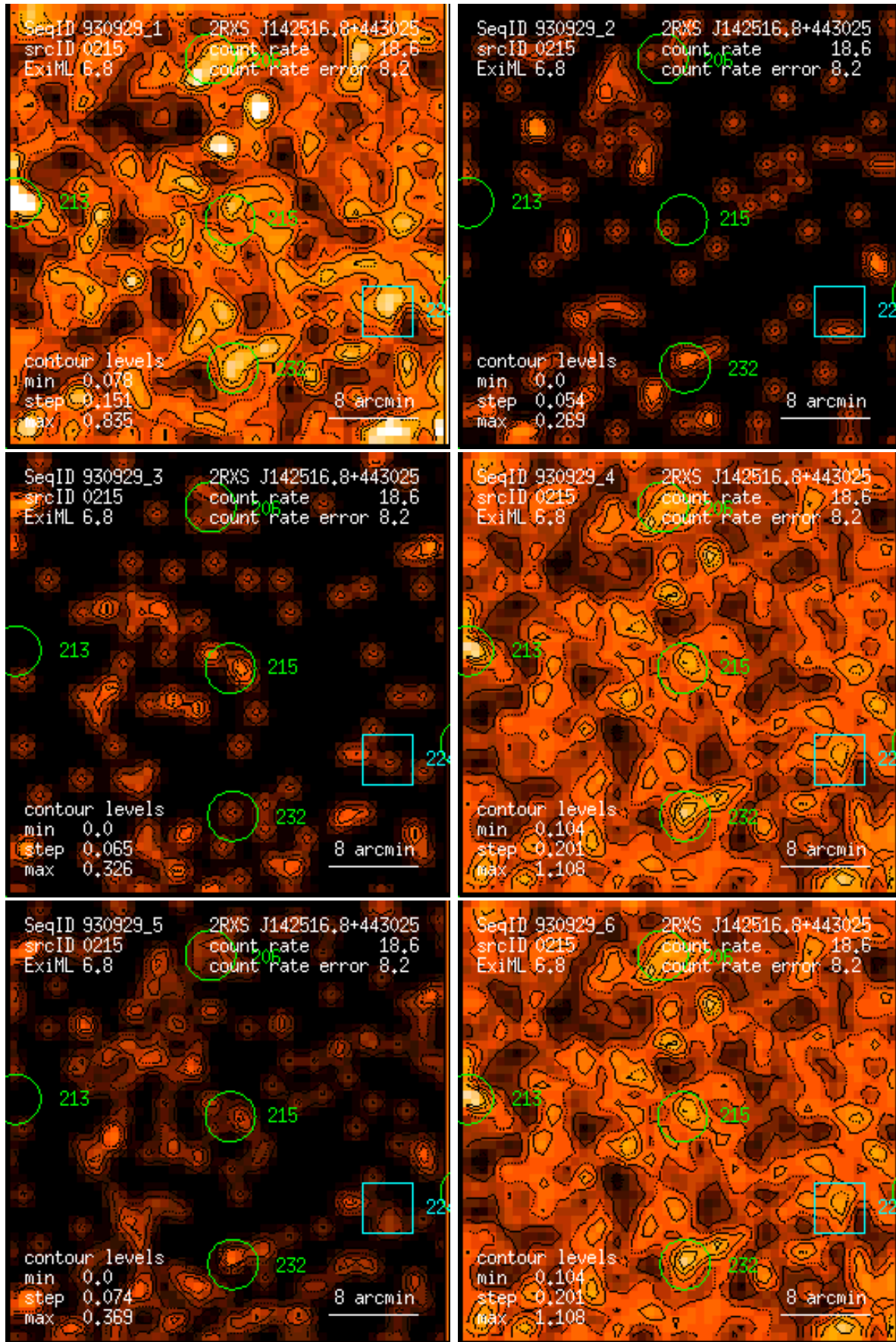
Figure 215: RASS 930929: detection 0215: band rate images, Gaussian filter: (1) PSPC channels 11 – 41, (2) 52 – 90, (3) 91 – 201, (4) 11 – 235, (5) 52 – 201, (6) 11 – 201. Broad band rates in counts/ks. Band rate contour levels in counts/ks/arcmin 2 .
