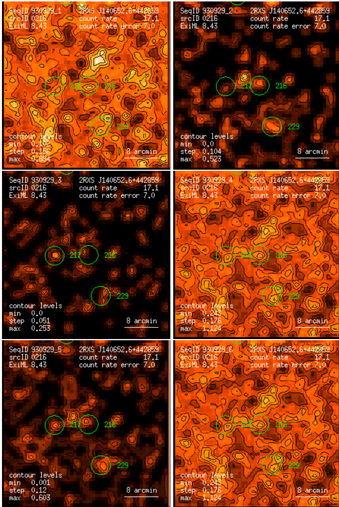
Figure 216: RASS 930929: detection 0216: band rate images, Gaussian filter: (1) PSPC channels 11 – 41, (2) 52 – 90, (3) 91 – 201, (4) 11 – 235, (5) 52 – 201, (6) 11 – 201. Broad band rates in counts/ks. Band rate contour levels in counts/ks/arcmin 2 .
