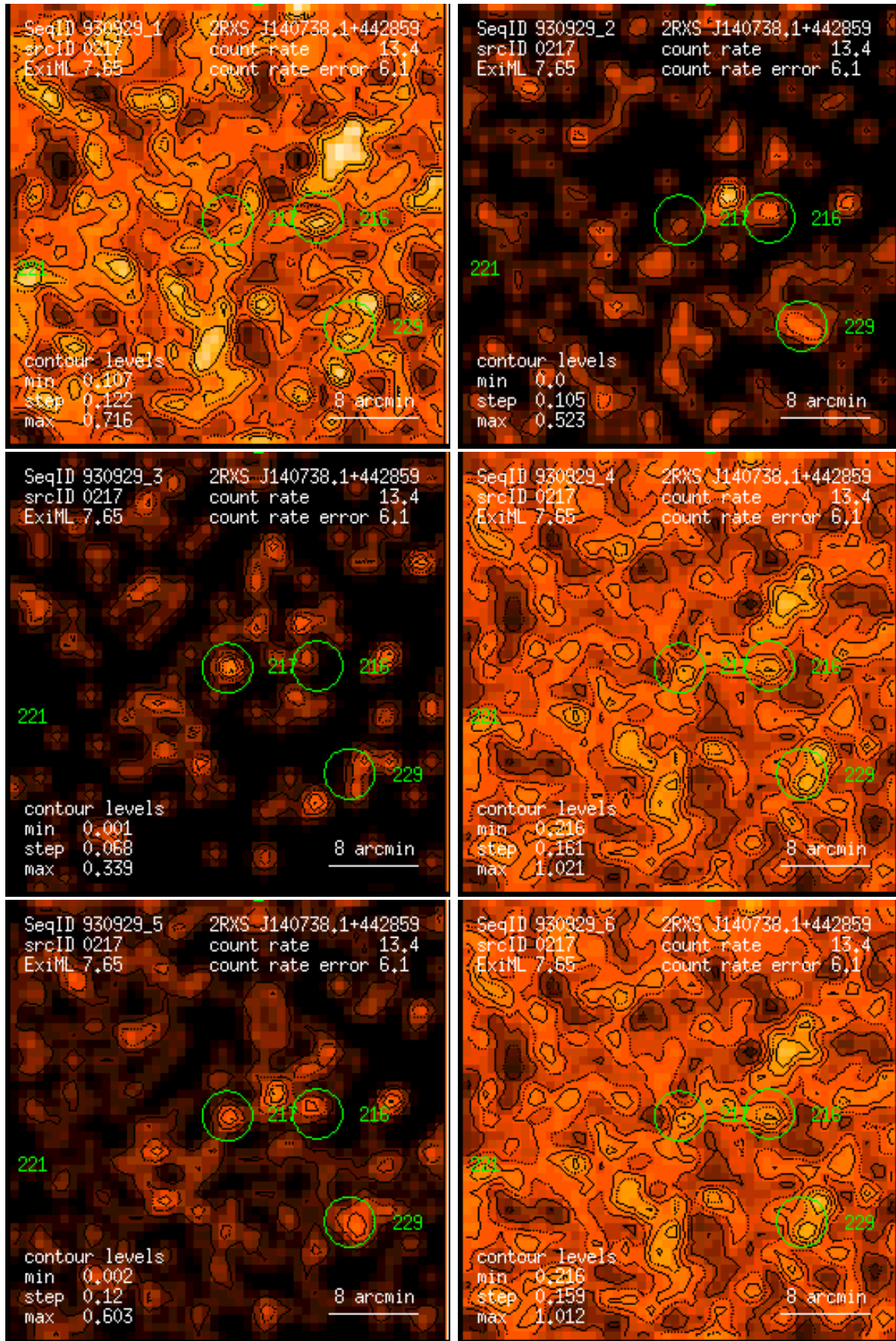
Figure 217: RASS 930929: detection 0217: band rate images, Gaussian filter: (1) PSPC channels 11 – 41, (2) 52 – 90, (3) 91 – 201, (4) 11 – 235, (5) 52 – 201, (6) 11 – 201. Broad band rates in counts/ks. Band rate contour levels in counts/ks/arcmin 2 .
