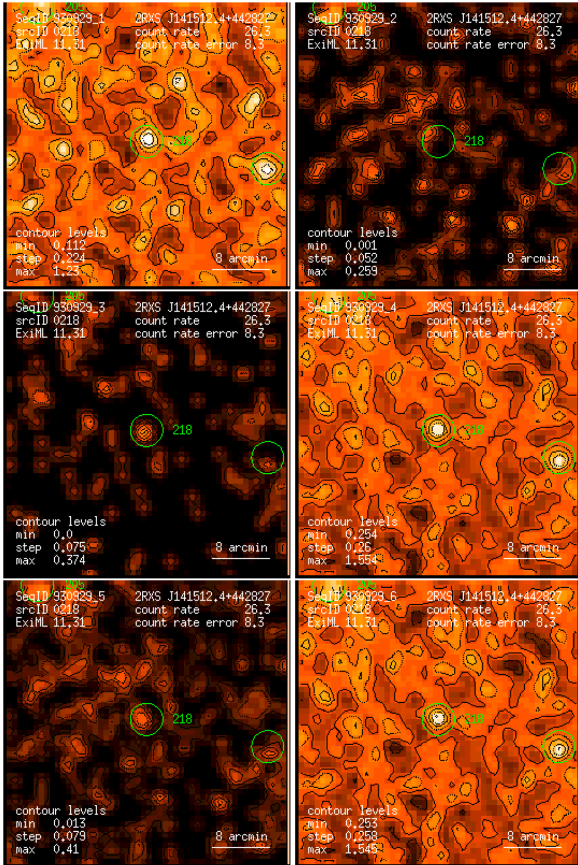
Figure 218: RASS 930929: detection 0218: band rate images, Gaussian filter: (1) PSPC channels 11 – 41, (2) 52 – 90, (3) 91 – 201, (4) 11 – 235, (5) 52 – 201, (6) 11 – 201. Broad band rates in counts/ks. Band rate contour levels in counts/ks/arcmin 2 .
