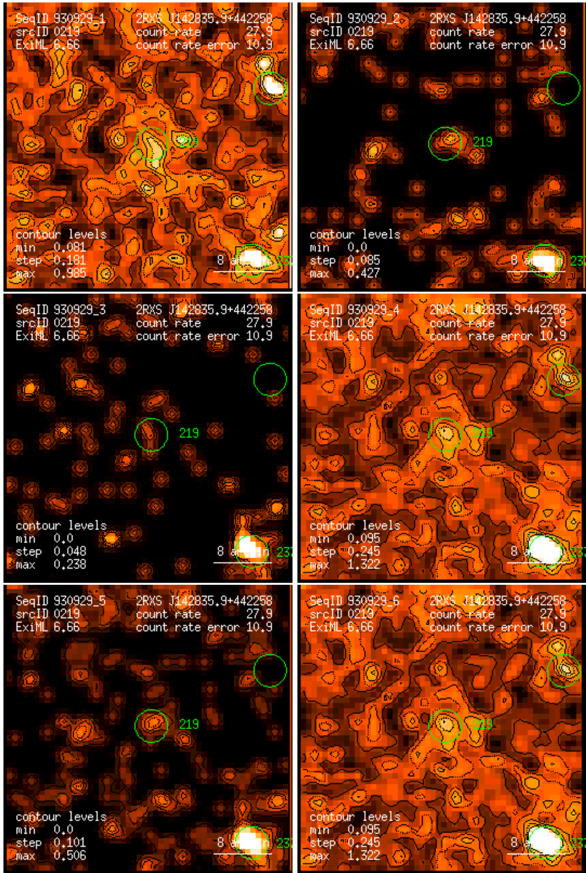
Figure 219: RASS 930929: detection 0219: band rate images, Gaussian filter: (1) PSPC channels 11 – 41, (2) 52 – 90, (3) 91 – 201, (4) 11 – 235, (5) 52 – 201, (6) 11 – 201. Broad band rates in counts/ks. Band rate contour levels in counts/ks/arcmin 2 .
