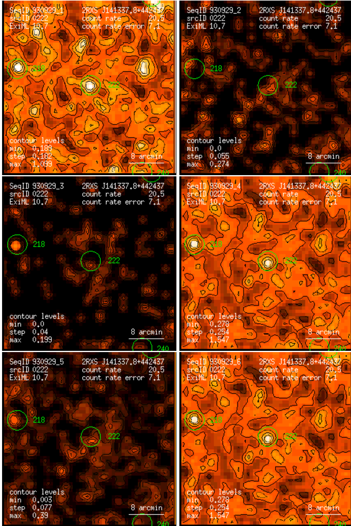
Figure 222: RASS 930929: detection 0222: band rate images, Gaussian filter: (1) PSPC channels 11 – 41, (2) 52 – 90, (3) 91 – 201, (4) 11 – 235, (5) 52 – 201, (6) 11 – 201. Broad band rates in counts/ks. Band rate contour levels in counts/ks/arcmin 2 .
