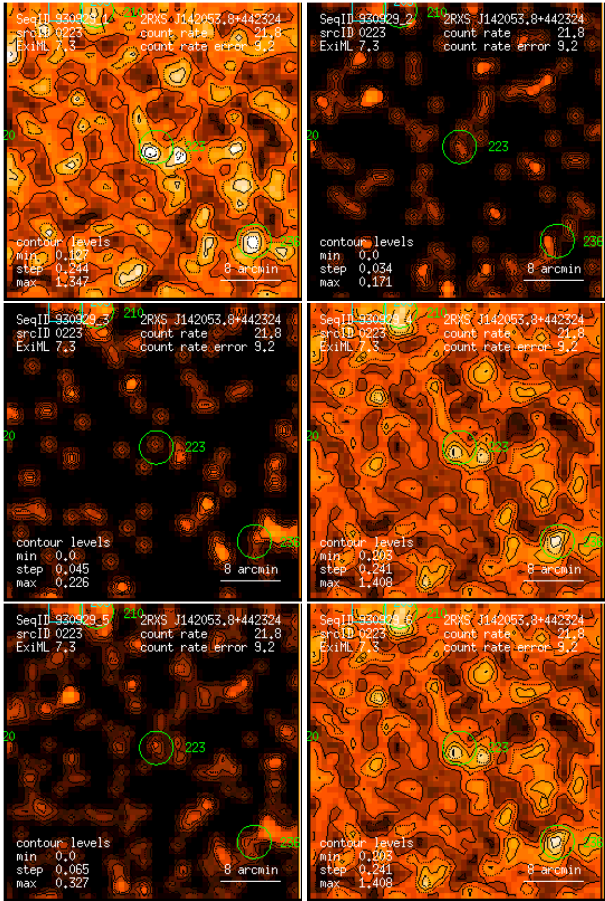
Figure 223: RASS 930929: detection 0223: band rate images, Gaussian filter: (1) PSPC channels 11 – 41, (2) 52 – 90, (3) 91 – 201, (4) 11 – 235, (5) 52 – 201, (6) 11 – 201. Broad band rates in counts/ks. Band rate contour levels in counts/ks/arcmin 2 .
