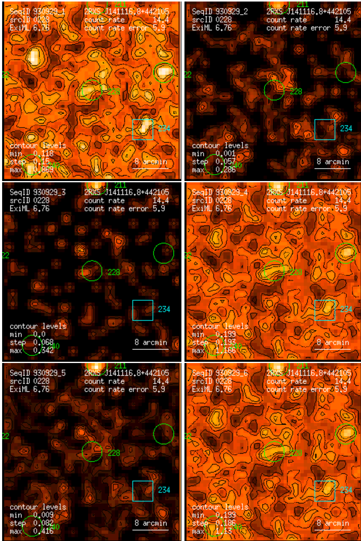
Figure 228: RASS 930929: detection 0228: band rate images, Gaussian filter: (1) PSPC channels 11 – 41, (2) 52 – 90, (3) 91 – 201, (4) 11 – 235, (5) 52 – 201, (6) 11 – 201. Broad band rates in counts/ks. Band rate contour levels in counts/ks/arcmin 2 .
