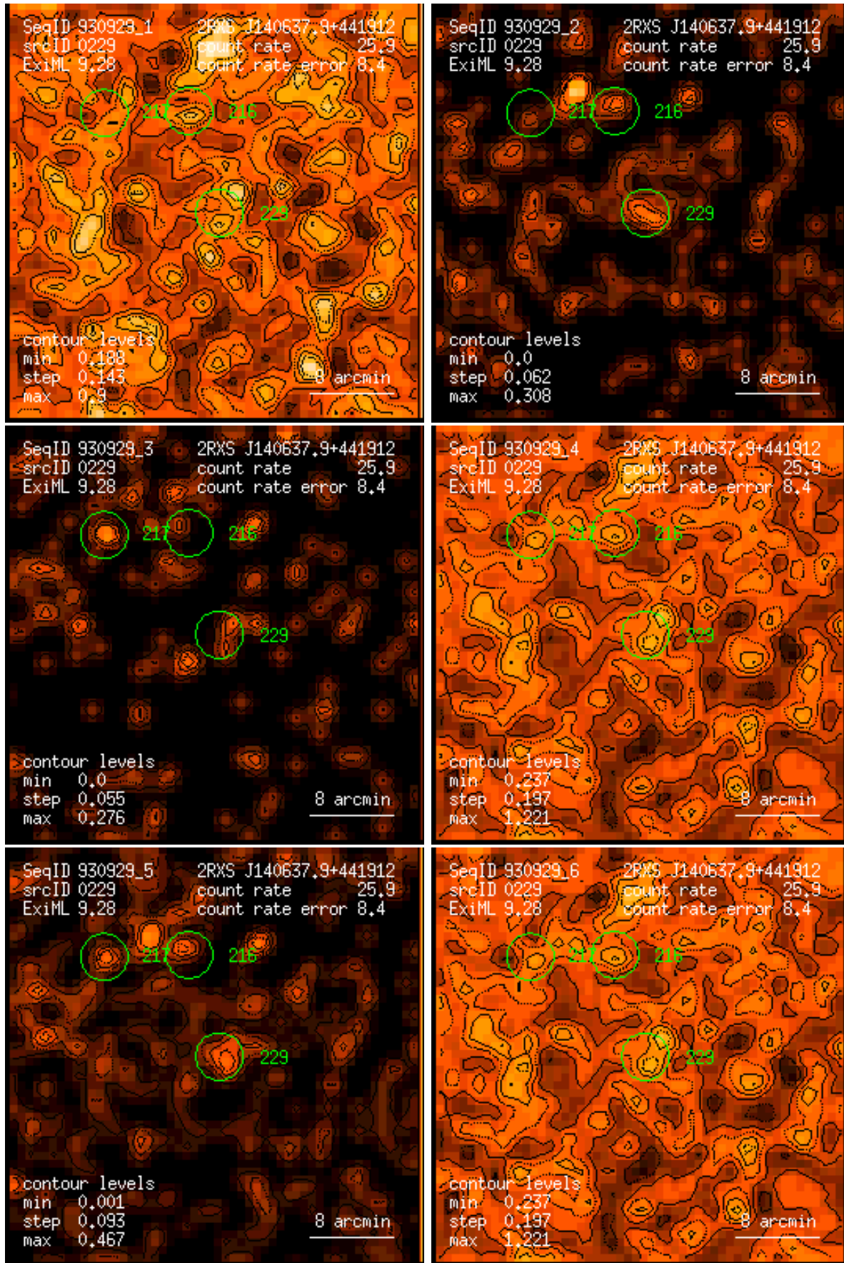
Figure 229: RASS 930929: detection 0229: band rate images, Gaussian filter: (1) PSPC channels 11 – 41, (2) 52 – 90, (3) 91 – 201, (4) 11 – 235, (5) 52 – 201, (6) 11 – 201. Broad band rates in counts/ks. Band rate contour levels in counts/ks/arcmin 2 .
