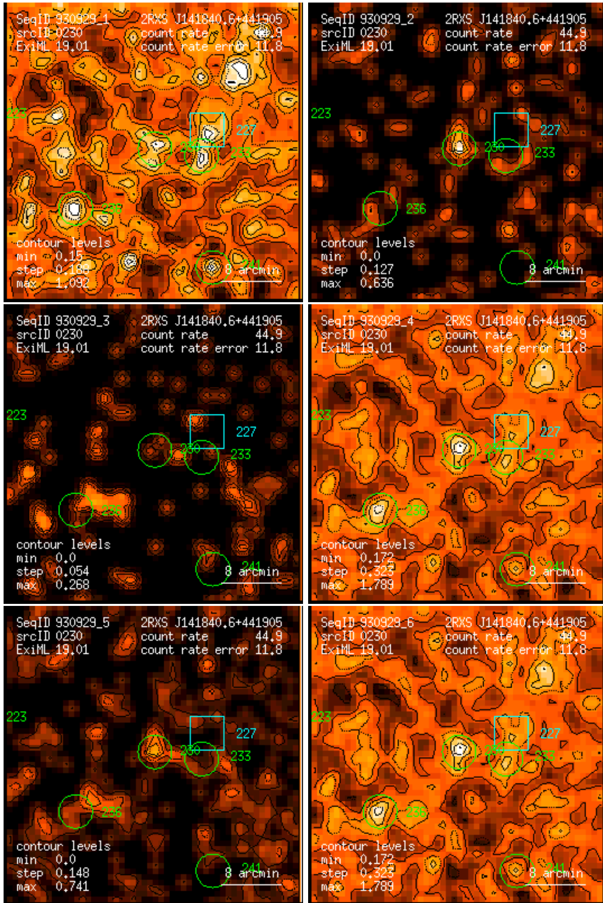
Figure 230: RASS 930929: detection 0230: band rate images, Gaussian filter: (1) PSPC channels 11 – 41, (2) 52 – 90, (3) 91 – 201, (4) 11 – 235, (5) 52 – 201, (6) 11 – 201. Broad band rates in counts/ks. Band rate contour levels in counts/ks/arcmin 2 .
