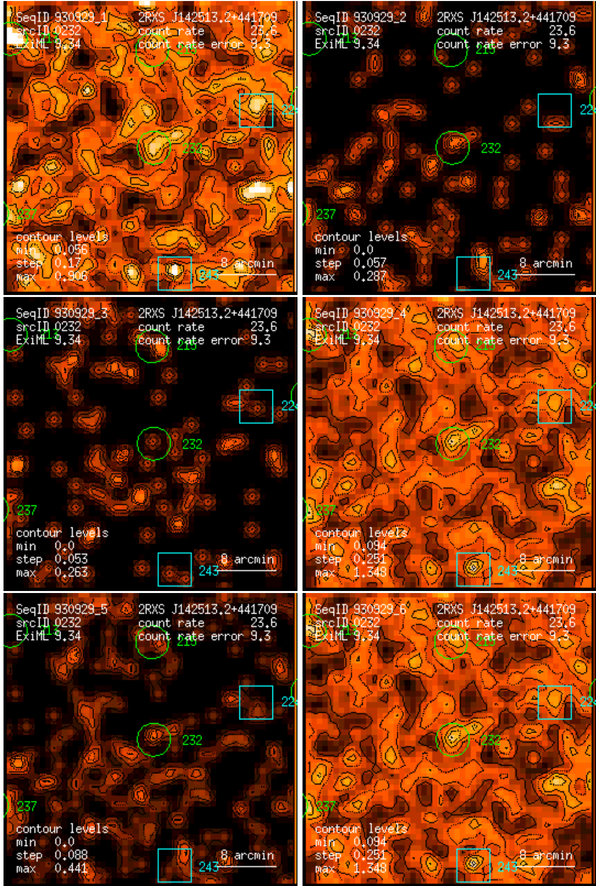
Figure 232: RASS 930929: detection 0232: band rate images, Gaussian filter: (1) PSPC channels 11 – 41, (2) 52 – 90, (3) 91 – 201, (4) 11 – 235, (5) 52 – 201, (6) 11 – 201. Broad band rates in counts/ks. Band rate contour levels in counts/ks/arcmin 2 .
