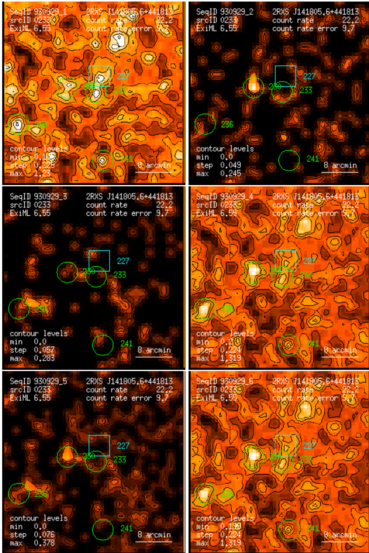
Figure 233: RASS 930929: detection 0233: band rate images, Gaussian filter: (1) PSPC channels 11 – 41, (2) 52 – 90, (3) 91 – 201, (4) 11 – 235, (5) 52 – 201, (6) 11 – 201. Broad band rates in counts/ks. Band rate contour levels in counts/ks/arcmin 2 .
