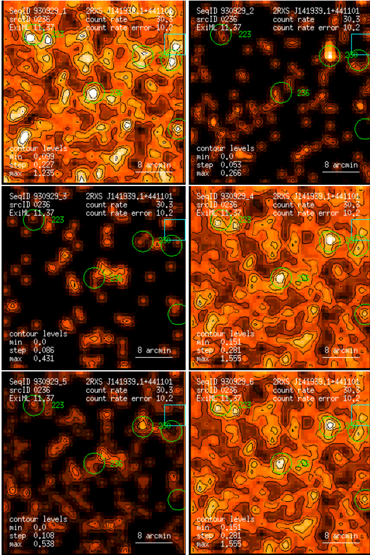
Figure 236: RASS 930929: detection 0236: band rate images, Gaussian filter: (1) PSPC channels 11 – 41, (2) 52 – 90, (3) 91 – 201, (4) 11 – 235, (5) 52 – 201, (6) 11 – 201. Broad band rates in counts/ks. Band rate contour levels in counts/ks/arcmin 2 .
