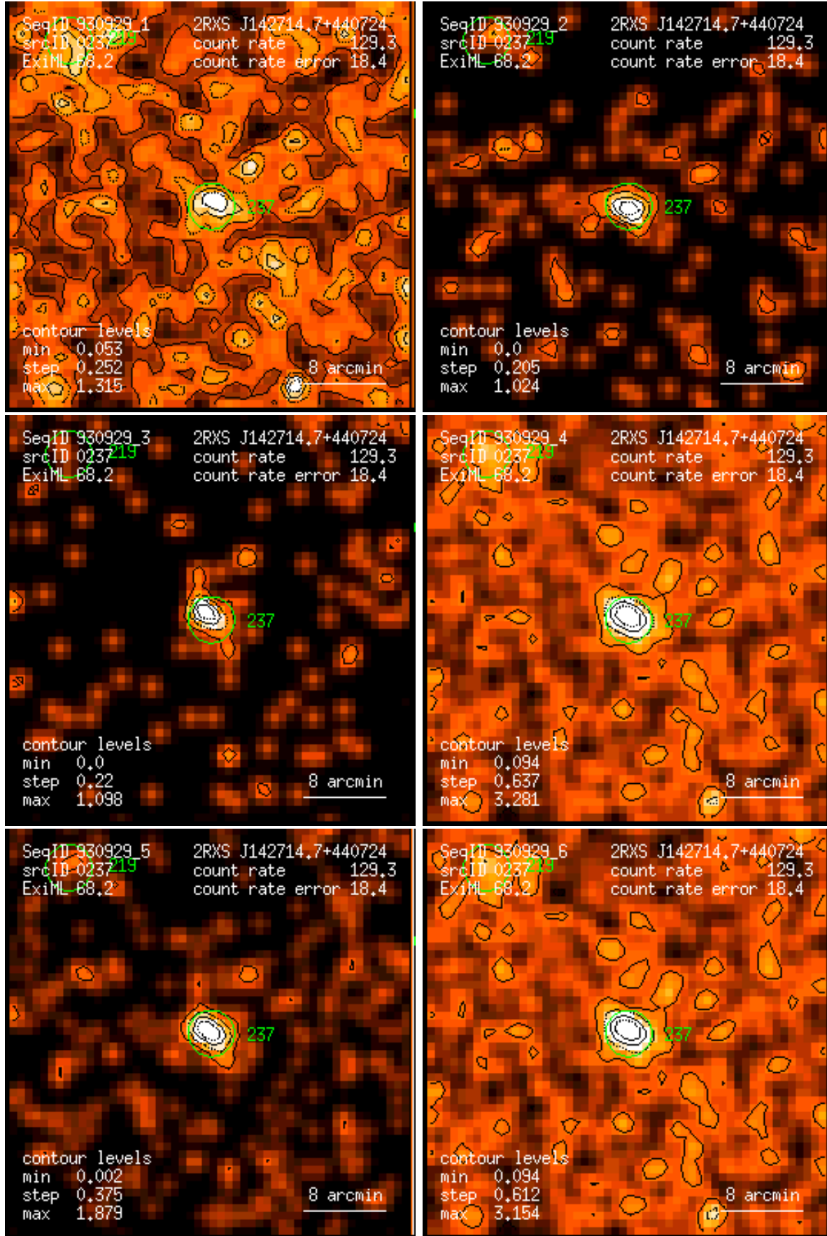
Figure 237: RASS 930929: detection 0237: band rate images, Gaussian filter: (1) PSPC channels 11 – 41, (2) 52 – 90, (3) 91 – 201, (4) 11 – 235, (5) 52 – 201, (6) 11 – 201. Broad band rates in counts/ks. Band rate contour levels in counts/ks/arcmin 2 .
