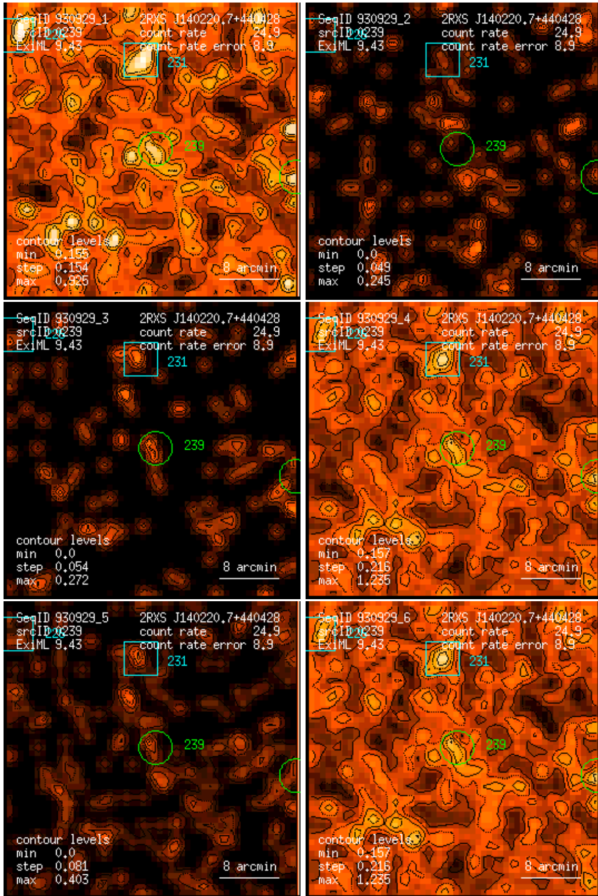
Figure 239: RASS 930929: detection 0239: band rate images, Gaussian filter: (1) PSPC channels 11 – 41, (2) 52 – 90, (3) 91 – 201, (4) 11 – 235, (5) 52 – 201, (6) 11 – 201. Broad band rates in counts/ks. Band rate contour levels in counts/ks/arcmin 2 .
