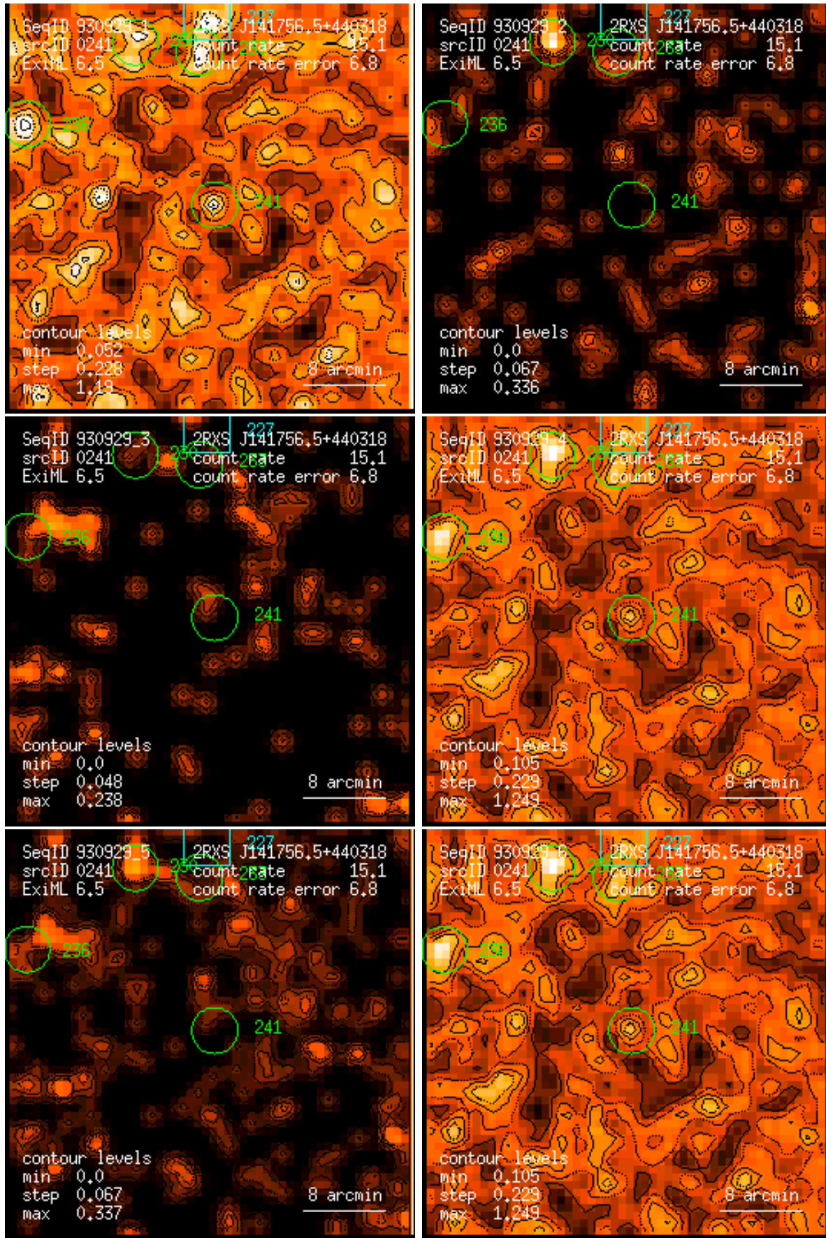
Figure 241: RASS 930929: detection 0241: band rate images, Gaussian filter: (1) PSPC channels 11 – 41, (2) 52 – 90, (3) 91 – 201, (4) 11 – 235, (5) 52 – 201, (6) 11 – 201. Broad band rates in counts/ks. Band rate contour levels in counts/ks/arcmin 2 .
