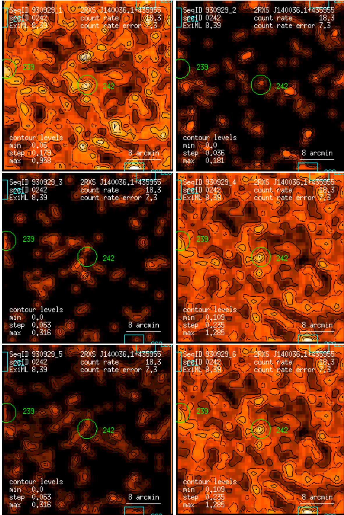
Figure 242: RASS 930929: detection 0242: band rate images, Gaussian filter: (1) PSPC channels 11 – 41, (2) 52 – 90, (3) 91 – 201, (4) 11 – 235, (5) 52 – 201, (6) 11 – 201. Broad band rates in counts/ks. Band rate contour levels in counts/ks/arcmin 2 .
