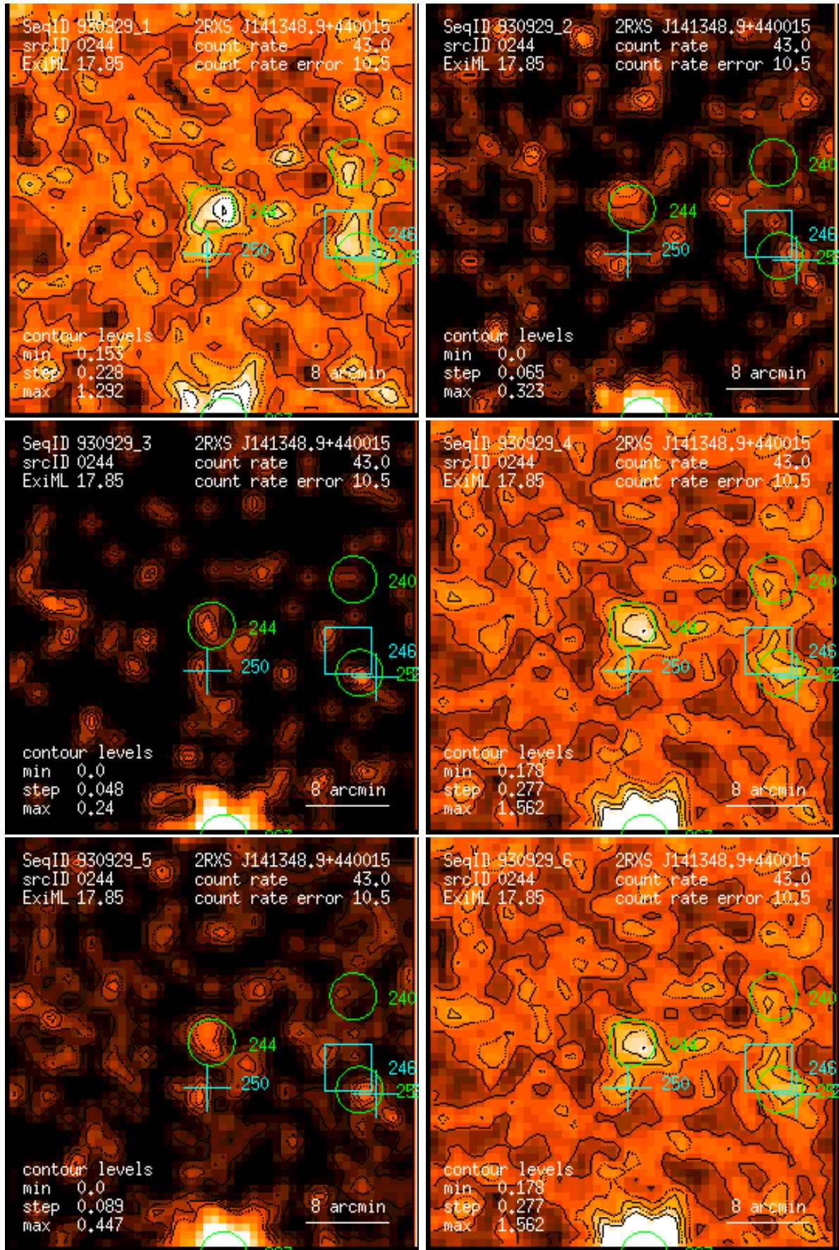
Figure 244: RASS 930929: detection 0244: band rate images, Gaussian filter: (1) PSPC channels 11 – 41, (2) 52 – 90, (3) 91 – 201, (4) 11 – 235, (5) 52 – 201, (6) 11 – 201. Broad band rates in counts/ks. Band rate contour levels in counts/ks/arcmin 2 .
