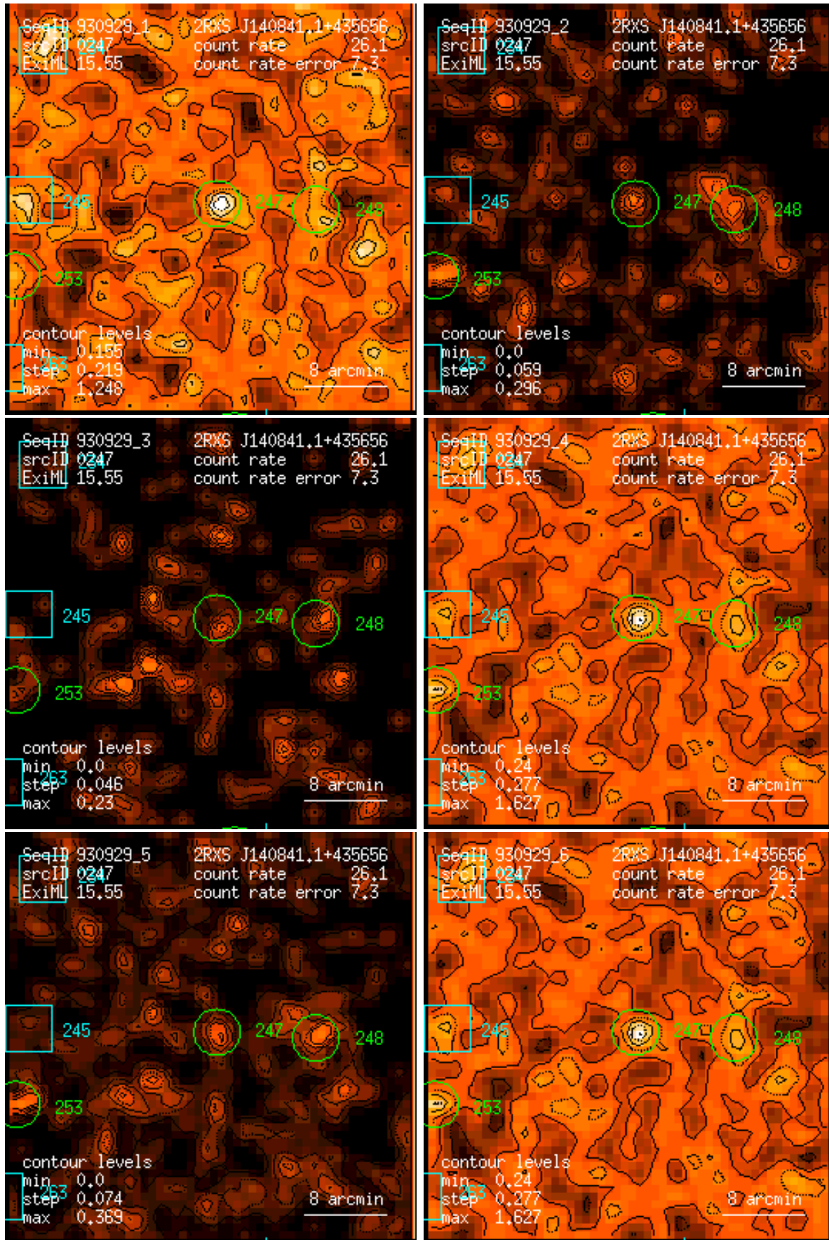
Figure 247: RASS 930929: detection 0247: band rate images, Gaussian filter: (1) PSPC channels 11 – 41, (2) 52 – 90, (3) 91 – 201, (4) 11 – 235, (5) 52 – 201, (6) 11 – 201. Broad band rates in counts/ks. Band rate contour levels in counts/ks/arcmin 2 .
